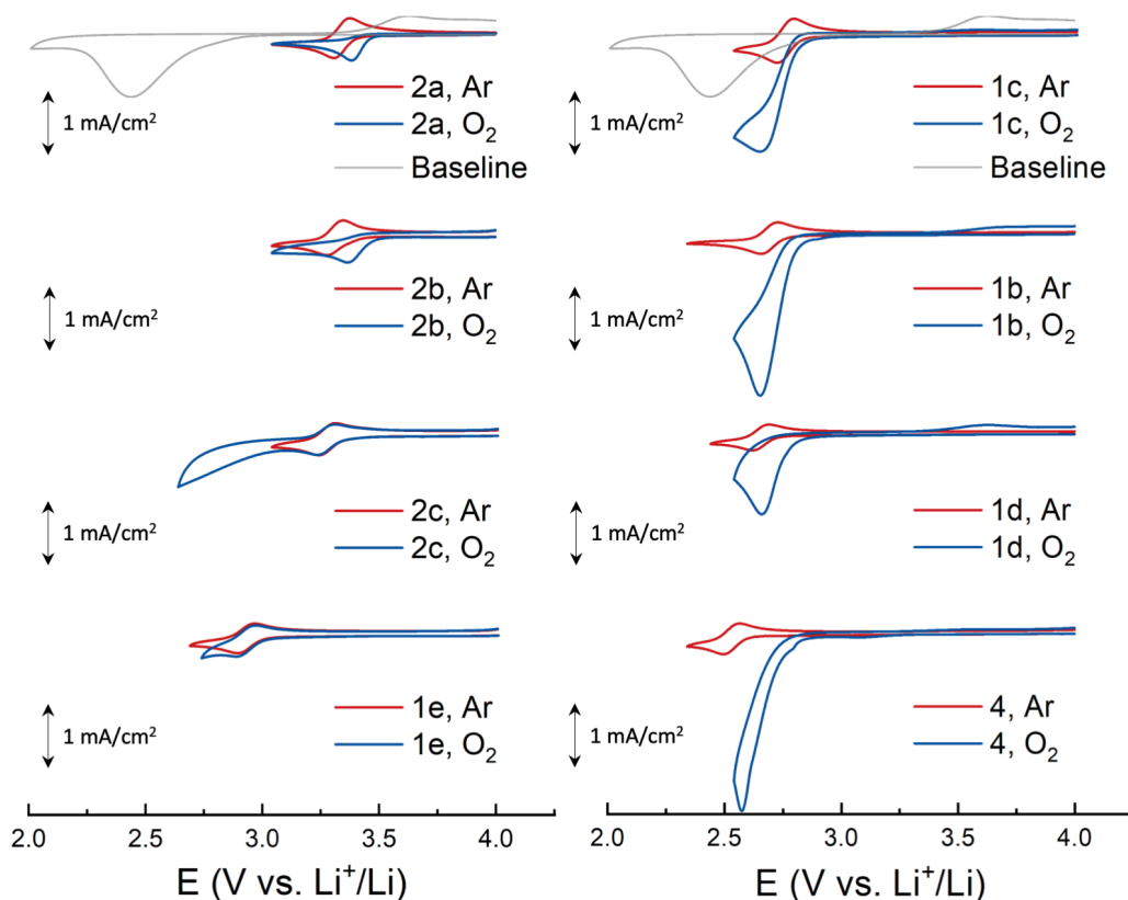
Figure 3. Cyclic voltammograms of redox mediators showing their effect on oxygen reduction in Li-O_2 cells. CVs of redox mediators in Ar - (red trace) and O_2 -saturated (blue trace) electrolyte and redox mediator-free solutions (grey) are shown. CVs were recorded in ACN containing 0.1 M tetrabutylammonium perchlorate (TBAP), 10 mM lithium triflate ( LiOTf ), and 1 mM redox mediator at the scan rate of 100 mV/s.
