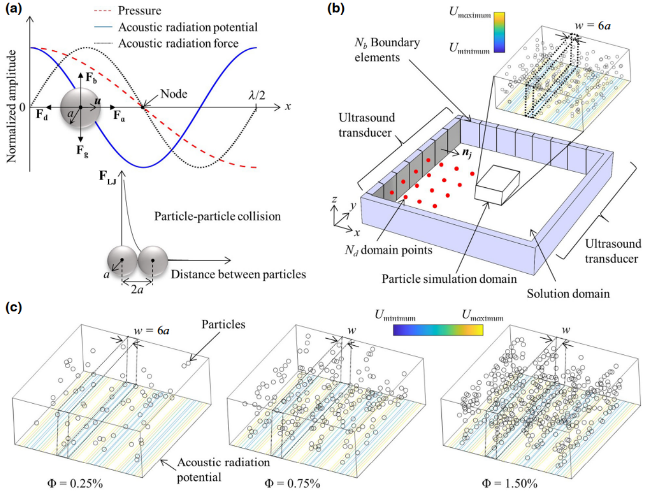
FIG. 1. (a) Schematic of a spherical particle in a viscous medium, and in a standing ultrasound wave field during ultrasound DSA, indicating the different forces acting on the particle. (b) Schematic of the 3D theoretical model of the reservoir with two ultrasound transducers affixed to opposing walls that contains the mixture of spherical particles dispersed in the viscous medium, showing the solution domain within a simply closed boundary. (c) Simulated 3D particle location for different particle volume fractions.
