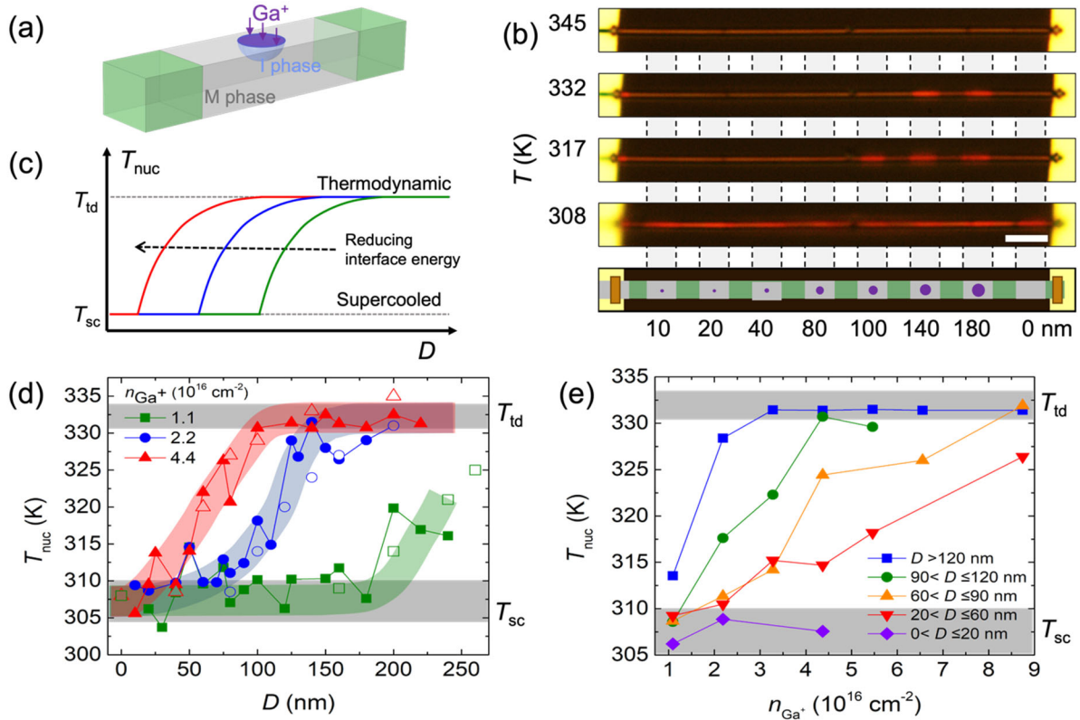
Figure 2: I-phase nucleation in supercooled VO 2 . (a) Schematic showing a disk-shaped nucleation seed (purple) created by Ga + ion irradiation on the surface of a shielded pristine VO 2 segment. The Ga + ion penetration depth is \sim 15 \text{ nm} , very shallow compared to the diameter of the irradiated area, hence the nucleation can be approximated as a disk shape with zero thickness. (b) Optical image of the I-phase nucleation process along a long, suspended VO 2 nanobeam. The nanobeam is divided into eight pristine segments, each shielded by two He + -irradiated segments; then a nucleation seed is introduced onto the surface of each of the pristine segments by Ga + irradiation at a dose of 2.2 \times 10^{16} \text{ ions/cm}^2 , but with different diameters. The lowest panel shows schematically the case where the diameter of the disk-shaped nucleation seed ( D ) increases from 10 to 180 nm. Scale bar is 5 \mu\text{m} . (c) Schematic dependence of I-phase nucleation temperature ( T_{\text{nuc}} ) on D , as predicted by classical nucleation theory. T_{\text{nuc}} is upper-bounded by the thermodynamic MIT temperature ( T_{\text{td}} ) and lower-bounded by the supercooled temperature ( T_{\text{sc}} ) of the shielded VO 2 . With reduced interface energy, stable nuclei with smaller D are able to form at a given temperature. (d) Measured (solid symbols) and calculated (open symbols) T_{\text{nuc}} as a function of D for different Ga + irradiation doses. The thick curved bands are a guide for the eye. The critical sizes of the nucleus can be determined from the onset of the rise above the supercooled limit. (e) Measured dependence of T_{\text{nuc}} on Ga + irradiation dose ( n_{\text{Ga}^+} ) in the seed at different D intervals. A heavier dose in the seed promotes I-phase nucleation as shown by the increased T_{\text{nuc}} . T_{\text{nuc}} for nucleation seeds with large D and high doses is found to reach the thermodynamic limit. T_{\text{td}} and T_{\text{sc}} are marked by the grey shaded areas in (d) and (e).
