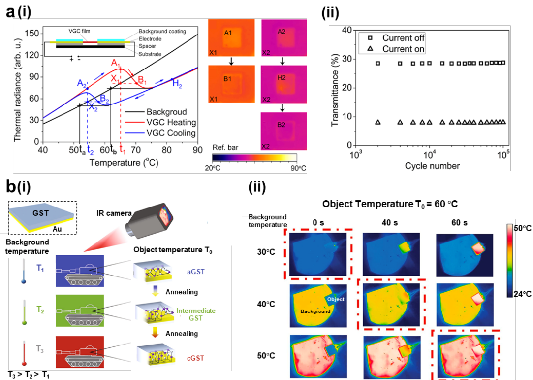
Figure 21. IR camouflage based on PCMs. (a) An adaptive thermal camouflage based on electrically heated VGC nano-thickness sandwich structure. (i) Left: the thermal radiance of the background coating (black line) and the VGC film (heating, red curve; cooling, blue curve); inset: the structure of the electrically tunable VGC-based device; right: thermal images of camouflage processes by direct (A1 –
