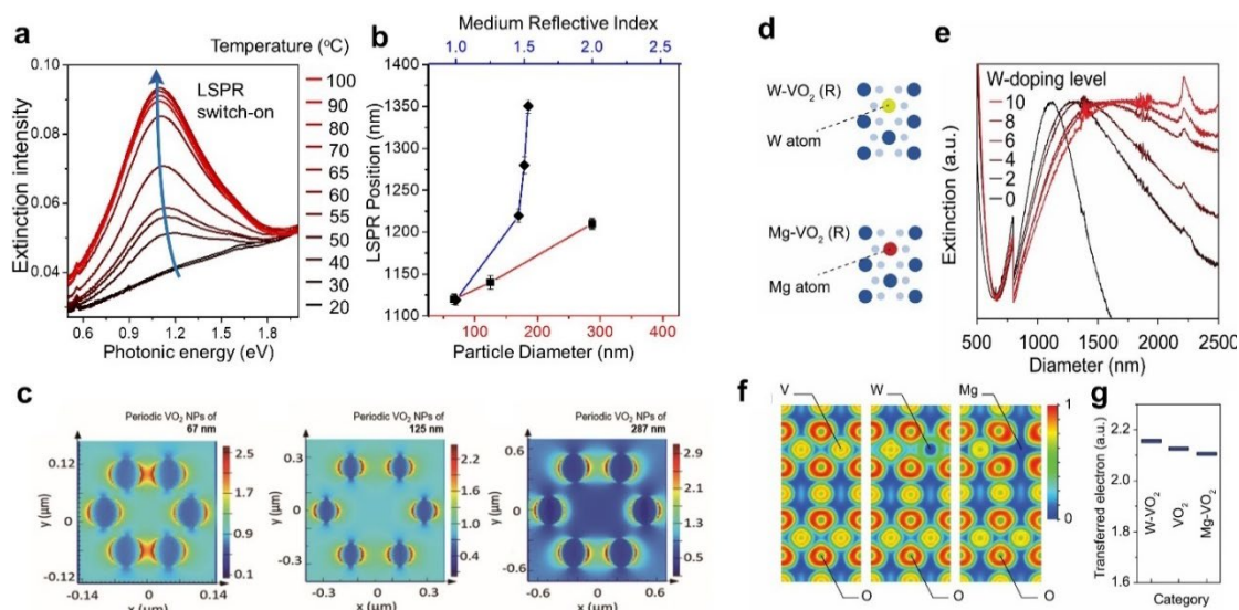
Figure 3. Modulation of LSPR in VO 2 . (a) The “on-off LSPR” behavior in temperature-responsive VO 2 (M/R). The LSPR intensity increases under elevated temperatures. (b) The effects of particle size and medium reflective index on the LSPR peak position. (c) Calculated electrical fields in the x-y plane of patterned VO 2 (R) nanoparticles with a periodicity of 67, 125, and 287 nm, respectively. 93 Reproduced with permission from ref 93 . Copyright 2017 American Chemical Society. (d) Illustration of the substitutional W and Mg dopant in VO 2 (R) crystal lattices. (e) Extinction spectra of VO 2 (R) nanoparticles with different W doping levels. (f) Calculated electron localization function (ELF) maps and (g) the total transferred electrons from V to O atoms of pristine VO 2 , W-VO 2 , and Mg-doped VO 2 (Mg-VO 2 ). 99 Reproduced with permission from ref 99 . Copyright 2017 Royal Society of Chemistry.
