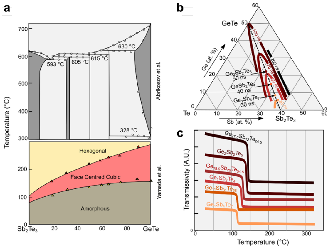
Figure 5. Properties of GeTe-Sb 2 Te 3 alloy. (a) The phase diagram for the GeTe-Sb 2 Te 3 pseudobinary (top panel) and the associated crystallization temperatures (bottom panel). 128 Reproduced with
