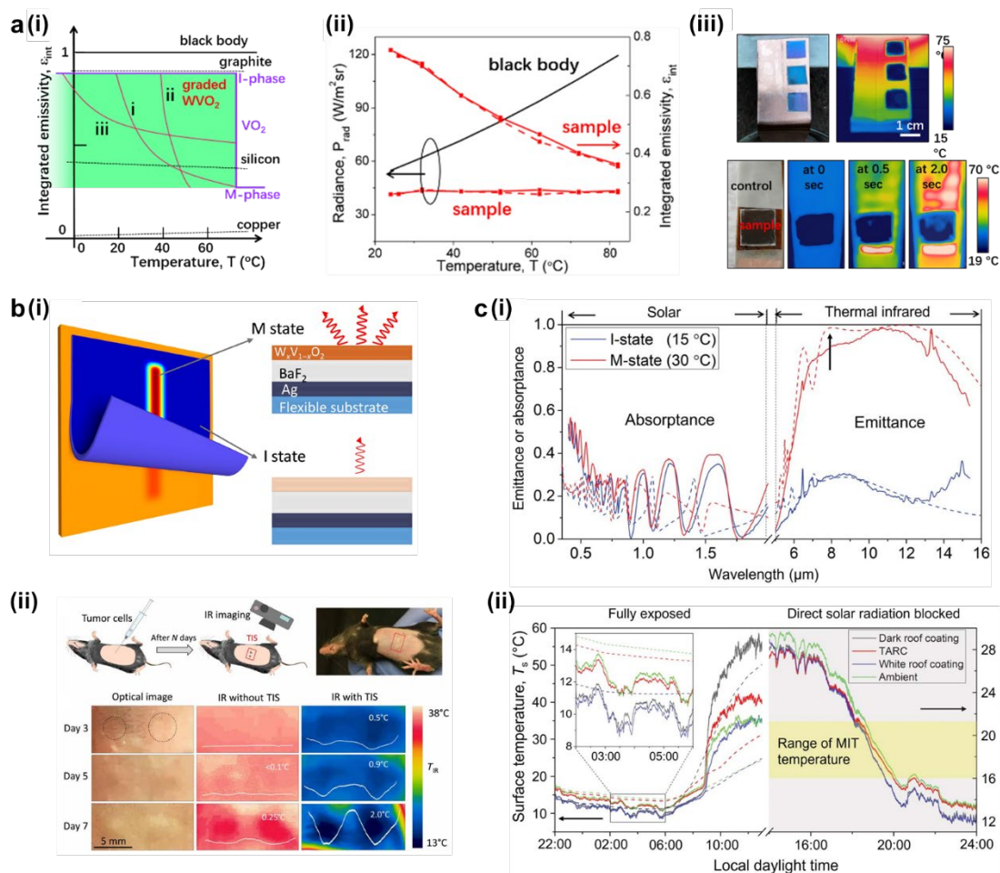
Figure 24. Thermal applications of W-VO 2 . (a) A thermal radiance modulation platform for advanced camouflage applications. (i) Schematics illustrating arbitrary realization of \epsilon(T) by graded doped W-VO 2 . (ii) Design of the \epsilon(T) to counteract the T^4 law, generating a temperature-independent thermal radiation power. (iii) Experiments demonstrating immunity of the camouflage to large spatial variation and a temporal surge of the surface temperature. 27 Reproduced with permission from ref 27 . Copyright 2020 Wiley-VCH. (b) TIS based on W-VO 2 . (i) Schematic illustration of boosted temperature resolution of thermography by TIS and its working mechanism. (ii) TIS applied to medical thermography, revealing early-stage tumors that are otherwise undetectable by conventional methods. 30 Reproduced with permission from ref 30 . Copyright 2020 American Association for the Advancement of Science under CC BY-NC 4.0. (c) A TARC for all-season household thermal regulation. (i) Solar spectral absorptance and part of the thermal spectral emissivity of TARC at I-state and M-state. (ii) Surface temperature of a TARC, a commercial dark roof coating ( A = 0.70 , \epsilon_w = 0.90 ), and a commercial white roof coating ( A = 0.15 , \epsilon_w = 0.90 ) in an open-space outdoor environment recorded over a day-night cycle. 32 Reproduced with permission from ref 32 . Copyright 2020 American Association for the Advancement of Science.
