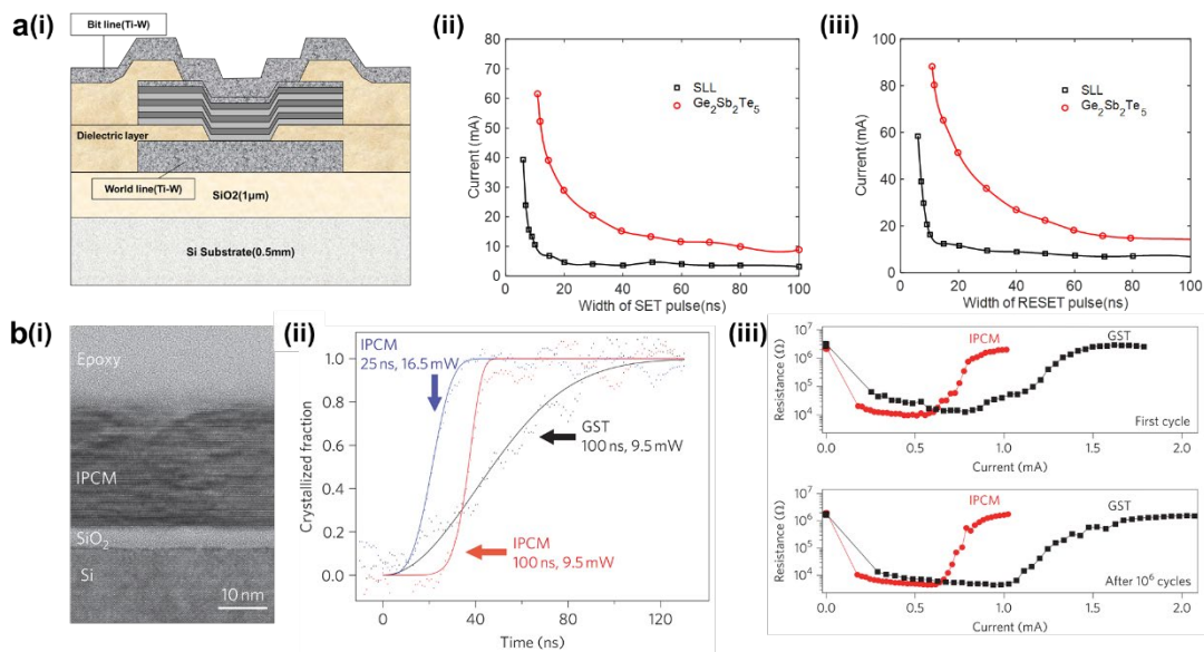
Figure 11. NVM based on SLL heterostructures. (a) A phase-change random access memory (PCRAM) cell with GeTe/Sb 2 Te 3 SLL structures. (i) Schematic diagram of the proposed cell structure. (ii) Comparison of the SET current versus pulse width between the SLL structure and the conventional GST material. (iii) Comparison of the RESET current versus pulse width between the SLL structure and the conventional GST material. 241 Reproduced with permission from ref 241 . Copyright 2006 American Institute of Physics. (b) An iPCM with GeTe/Sb 2 Te 3 heterostructures. (i) TEM image of the proposed (GeTe) 2 (Sb 2 Te 3 ) 4 interfacial phase-change material on a silicon substrate. (ii) The change of re-crystallized fraction versus time for GST (100 ns, 9.5 mW pump pulses; black); iPCM (100 ns, 9.5 mW pump pulses; red); iPCM (25 ns, 16.5 mW pump pulses; blue). (iii) Comparison of resistance change versus current between the iPCM and the GST-based cell in the first cycle (top) and after 1 × 10 6 cycles (bottom). 124 Reproduced with permission from ref 124 . Copyright 2011 Macmillan Publishers Limited.
