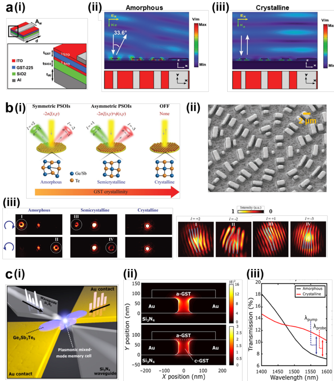
Figure 18. PCMs based plasmonic devices for phase control and waveguide memory. (a) Reconfigurable metasurfaces incorporated with PCM for beam steering. (i) Schematic showing the design of actively controlled beam steering. (ii) anomalous reflection ( \theta_r = 33.6^\circ ) with amorphous GST layer. (iii) Specular reflection with crystalline GST layer. 46 Reproduced with permission from ref 46 . Copyright 2018 Wiley-VCH. (b) Active switching of PSOs in phase-change metasurfaces. (i) The schematic diagram of active PSOs enabled by the proposed phase-change metasurfaces. (ii) SEM images of the fabricated metasurface consisting of top Au and GST nanobar deposited on Au film. (iii) Measured diffraction patterns at different crystallization levels under RCP and LCP illumination (left) and interference patterns obtained through the interference of the orbital angular momenta (OAM) beams and a tilted circularly polarized Gaussian beam (right). 370 Adapted with permission from ref 370 .
