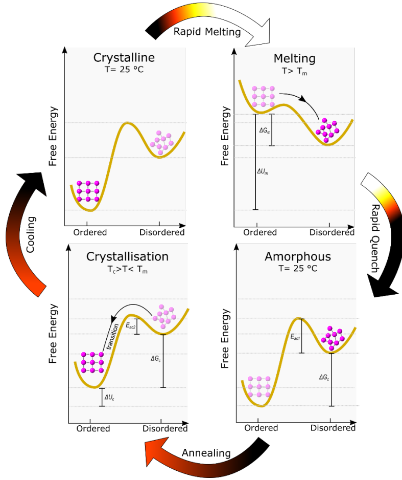
Figure 7. Changes in the potential landscape due to quenching and annealing \text{Sb}_2\text{Te}_3\text{-GeTe} PCM.
