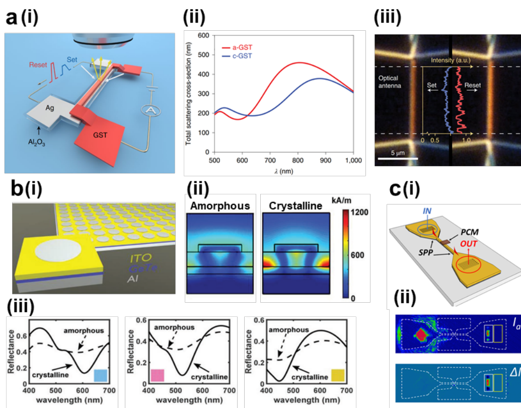
Figure 17. PCMs based plasmonic devices for intensity control. (a) Electrically tunable nano-antenna based on GST. (i) Schematic showing an optical antenna comprised of a GST nanobeam stacked on top of a silver nanostrip, separated by a thin Al 2 O 3 layer. (ii) The simulated total scattering cross-section of the optical antenna with a-GST and c-GST. (iii) Dark-field, white-light-scattering images of the antenna taken after a set pulse and a reset pulse, showing a notable change in the scattering intensity. The scattered light intensity measured along the antenna length is plotted in the inset. 353 Reproduced with permission from ref 353 . Copyright 2021 Springer Nature. (b) A phase-change metamaterial with the capability of nonvolatile color display. (i) 3D schematic of the phase-change MIM absorber structure and the materials used. (ii) Magnitude of the magnetic field (in the direction perpendicular to the plane) in the MIM absorber with the GeTe layer in the amorphous (left) and crystalline (right) phase. (iii) Optimized reflectance spectra of the cyan (left), magenta (middle), and yellow (right) pixels, as obtained by finite element method (FEM) simulation. 44 Reproduced with permission from ref 44 . Copyright 2019 Wiley-VCH. (c) Active control of surface plasmon waveguides.
