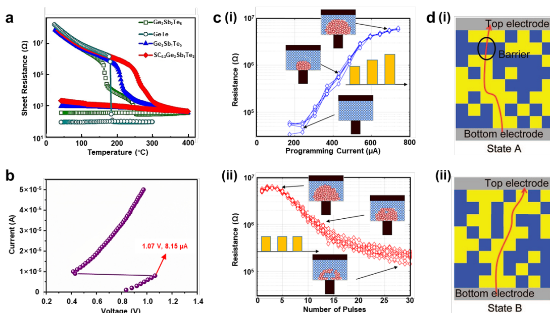
Figure 8. Electrical properties of PCMs. (a) The change of sheet resistance with different in situ annealing temperatures for the \text{GeTe} , \text{GST} , \text{Ge}_2\text{Sb}_1\text{Te}_2 , and \text{Sc}_{0.2}\text{Ge}_2\text{Sb}_1\text{Te}_2 films. 175 Reproduced with permission from ref 175 . Copyright 2019 Acta Materialia Inc. (b) I-V curve of the Sb-Ge SLL thin films. The threshold switching can be seen when the curve snaps back. 176 Reproduced with permission from ref 176 . Copyright 2017 Elsevier B.V. (c) Iterative RESET and cumulative SET process. (i) Possible achievable resistance values as a function of partial RESET pulses with varying amplitude. (ii) Evolution of resistance values versus the successive application of a SET pulse with the same amplitude. 177 Reproduced with permission from ref 177 . Copyright 2018 Creative Commons Attribution. (d) Schematic showing different mixed-phase configurations characterized by an incomplete (i) or complete (ii) percolation path through low-resistivity crystalline grains. The resistance is smaller in state A due to a small amorphous “barrier”. Yellow, crystalline; blue, amorphous. 33 Reproduced with permission from ref 33 . Copyright 2010 American Chemical Society.
