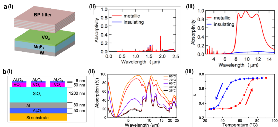
Figure 22. Self-adaptive radiative coolers based on VO 2 . (a) A proposed Fabry-Perot cavity structure based on VO 2 /MgF 2 /W, which is integrated with the top bandpass filter. (i) Schematic of the combined system of the Fabry-Perot cavity and bandpass filter. (ii) Solar and mid-IR (iii) absorptivity for M and I states are calculated. 380 Reproduced with permission from ref 380 . Copyright 2018 Optical Society of America. (d) A fabricated smart radiator by meta-surface of VO 2 . (i) Schematic showing the proposed VO 2 based metasurface for adaptive radiative cooling. (ii) Absorption spectra of the meta-reflector measured at 25, 40, 60, 70, and 80 °C. (iii) Emissivity change of the meta-reflector when the device is heated from 25 °C to 90 °C (blue) and then cooled down (red). A modulation magnitude of 0.43 can be measured for emissivity between the metal state and the insulator state. 397 Reproduced with permission from ref 397 . Copyright 2018 American Chemical Society.
