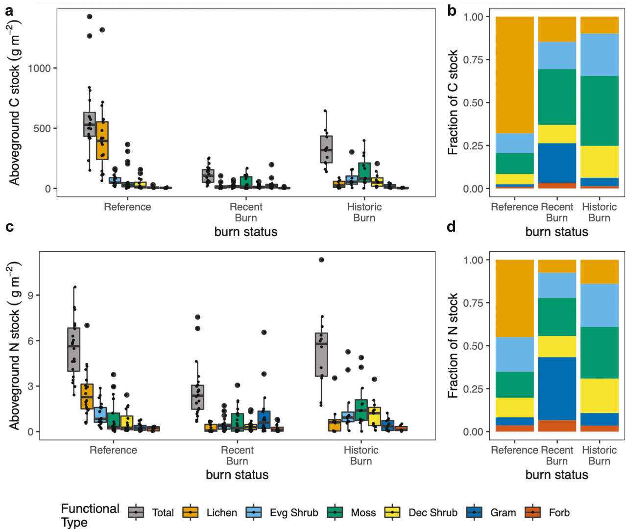
Figure 2. (a) Absolute and (b) mean relative within-treatment C stocks (or biomass) for each functional type and (c) absolute and (d) mean relative within-treatment N stocks. Points overlaid on box plots in (a) and (c) indicate the total C or N stock for a functional type in a single replicate plot. Box plot boundaries denote quartiles and medians, and whiskers denote 1.5 \times interquartile range. The corresponding significance of differences between burn treatments can be found in Table 2.
