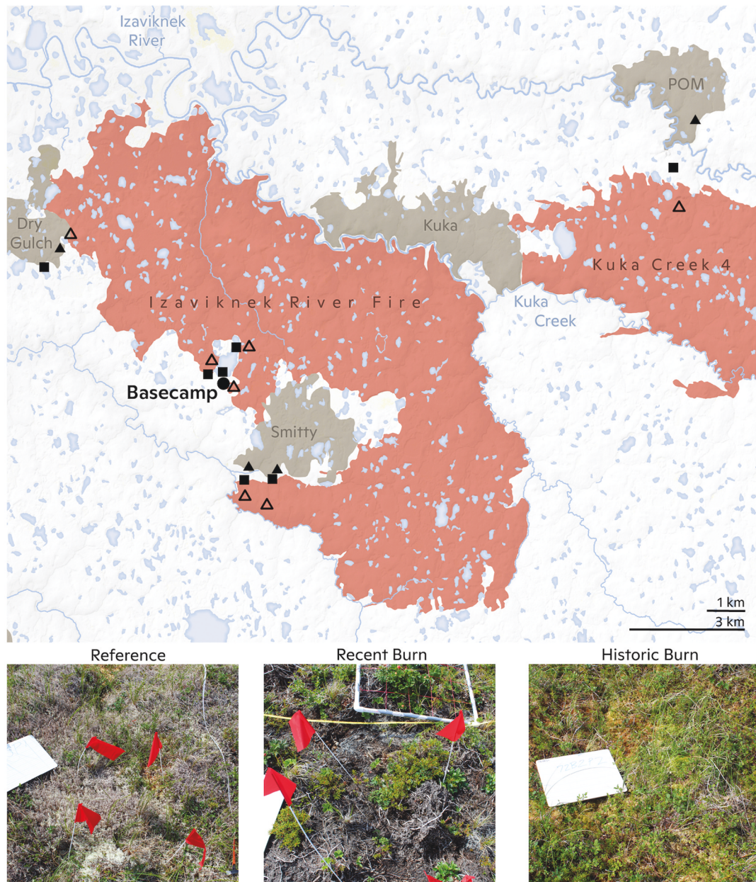
Figure 1. Map of burn history and sampled areas in the Yukon-Kuskokwim Delta (YKD) of Alaska. The bottom panel includes photos of plots sampled in reference, recent burn, and historic burn areas. Map created by Carl Churchill.
