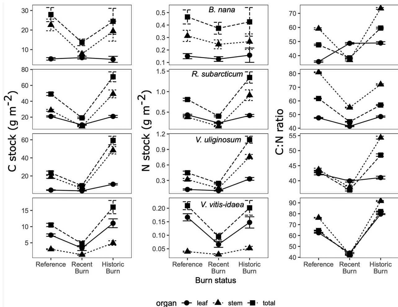
Figure 3. Carbon and N stocks and C:N of leaves (circle), stems (triangle), and whole plants (square) for four shrubs. Each row corresponds to the species denoted in the N stock column. Arithmetic mean and standard error are reported for C and N stocks, and geometric mean and standard deviation are reported for C:N.
