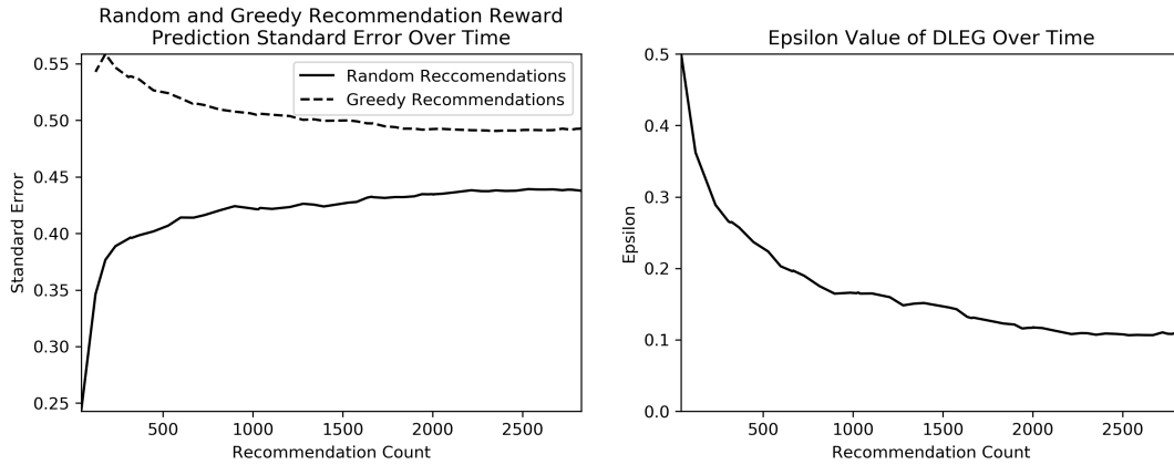
Figure 3: The standard error of the predictions made for random and greedy recommendations (left) and the resulting \epsilon (right) calculated by DLEG for the skill-level video study.
