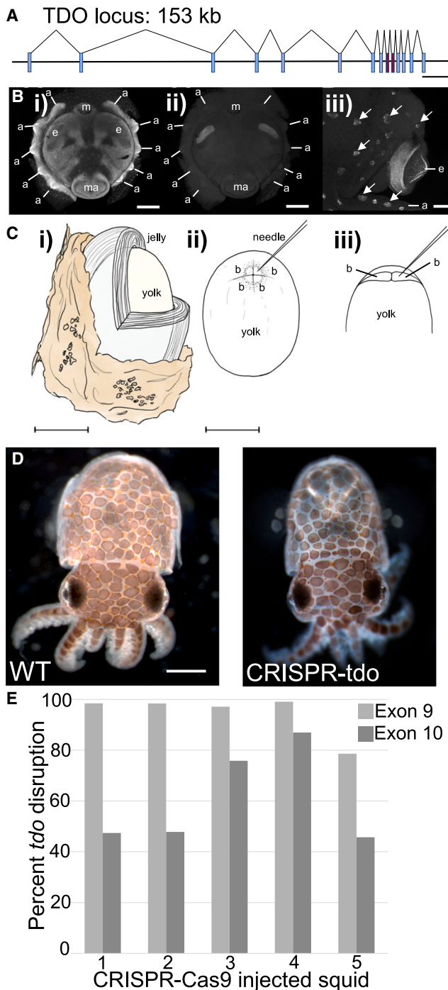
Figure 1. CRISPR-Cas9-mediated mutagenesis of TDO in E. berryi (A) Schematic of the E. berryi TDO locus showing 15 exons and 14 introns. gRNAs target exons 9 and 10 (red); scale bar, 10 kb. See also Figure S1.
