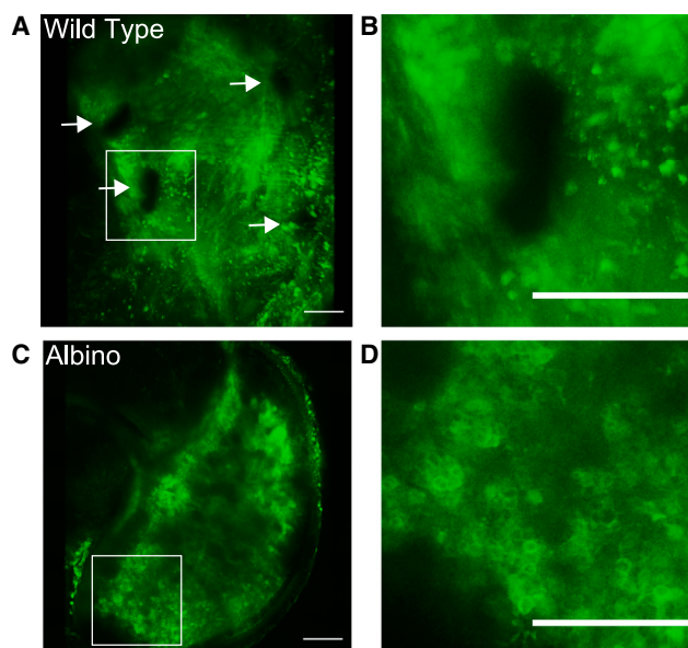
Figure 6. Albino squid provide clear optical access to optic lobes (A) The optic lobe of wild-type E. berryi was loaded with the calcium indicator Cal-520. The image was produced by maximum intensity projection of a 300 nm z stack. White arrows point to pigments on the skin surface that obstruct the image. Note the chromatophores were highly constricted during the experiment. (B) Magnified view of the white square in (A) is shown. (C and D) Same as in (A) and (B), but for albino E. berryi . Note a lack of black spots over the optic lobe that would have blocked the image and the presence of clear circular shapes that reflect successful imaging of the cells loaded with Cal-520. Scale bars, 100 \mu m.
