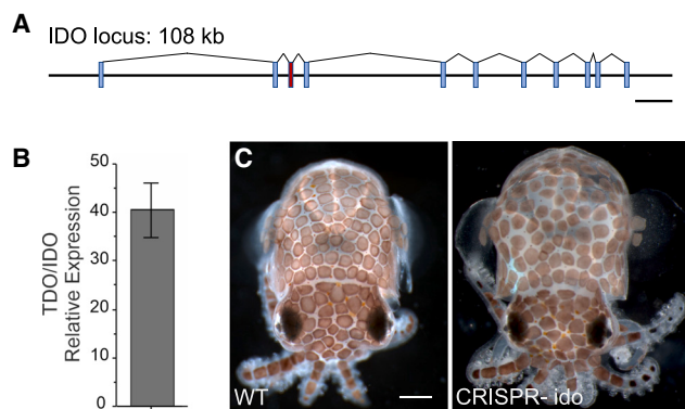
Figure 3. CRISPR-Cas9-mediated knockout of IDO in E. berryi
