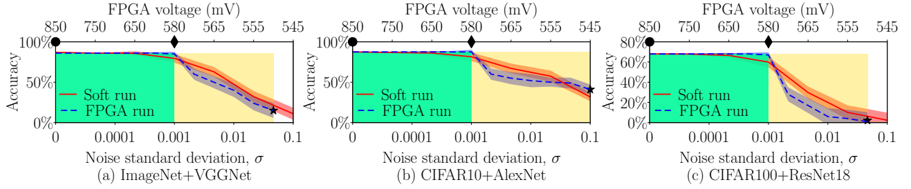
Fig. 3: Effects of stochastic noise and FPGA undervolting on utility or classification accuracy. ( V_{nom} : \circ , V_{min} : \blacklozenge , V_{crash} : \star ). V_{nom} , V_{min} , and V_{crash} are nominal, end of safe region, and start of crash region voltages, respectively.
