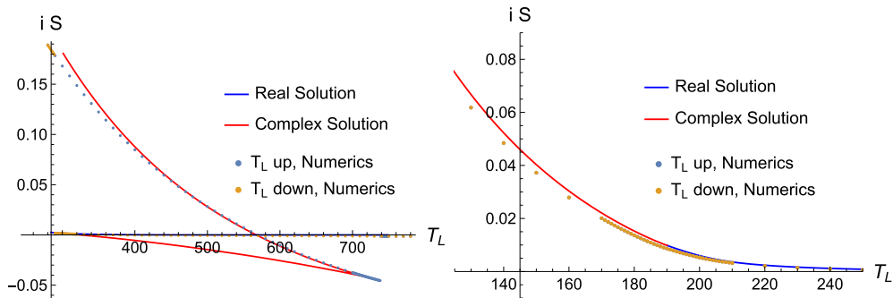
FIG. 7. Rate function iS in the large q limit with q = 96 and \mathcal{J} = 1 for (left) \hat{\mu} = 0.5 and (right) \hat{\mu} = 1.9 . For comparison, we also plot the numerical solutions of the saddle point equations (blue and orange dots).
