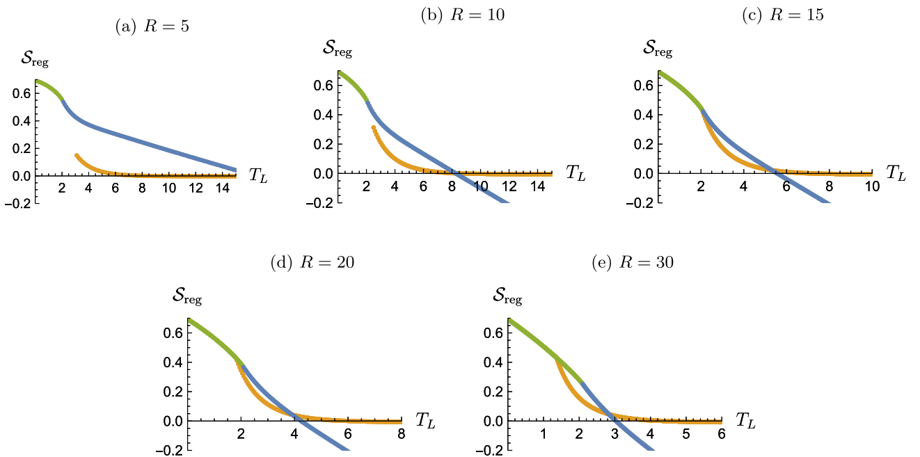
FIG. 11. Time evolution of the rate function in Eq. (52) for various values of the dissipative strength R ( q = 4, J = 1, K = 0.3 ).
