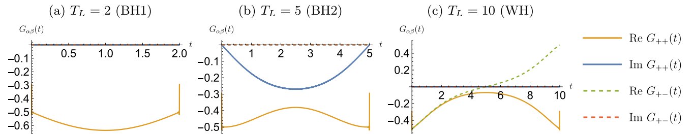
FIG. 9. Representative saddle point Green's functions G_{++}(t) and G_{+-}(t) in the SYK Lindbladian with the quadratic jump operators ( J = 1, K = 0.5 , and R = 2 ) for (a) black hole 1 (BH1) phase ( T_L = 2 ), (b) black hole 2 (BH2) phase ( T_L = 5 ), and (c) wormhole (WH) phase ( T_L = 10 ).
