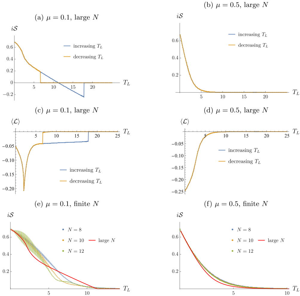
FIG. 1. Time evolution of the rate function (Loschmidt amplitude) iS of the SYK Lindbladian ( J = 1 ) with the nonrandom linear dissipators for (a) weak dissipation \mu = 0.1 and (b) strong dissipation \mu = 0.5 . We obtain the rate function by solving the large N saddle-point equation numerically by increasing (blue curve) and decreasing (orange curve) T_L . (a) In the weak-dissipation regime, the two saddle-point solutions are different from each other for 7 \lesssim T_L \lesssim 18 , which signals a discontinuous phase transition around T_L \approx 11 . The second-order derivative of the rate function iS is discontinuous around T_L \approx 2 , which corresponds to a continuous phase transition. (b) In the strong-dissipation regime, no dynamical quantum phase transitions occur. In (c) and (d), the derivatives of the rate functions are shown, which are equivalent to the expectation values \langle \mathcal{L} \rangle of the Lindbladians [see Eq. (25)]. In (e) and (f), comparisons with finite N results from exact diagonalization of the Lindbladian are presented for N = 8, 10, 12 , where the error bars show sample-to-sample fluctuations.
