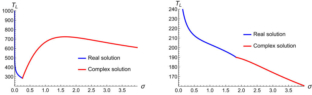
FIG. 6. T_L as a function of \sigma in the large q solutions for q = 96 . Left: For the weak dissipation \hat{\mu} = 0.5 , T_L is not a monotonic function of \sigma , and for fixed T_L , there are one real and two complex solutions in the intermediate regime. Right: For the strong dissipation \hat{\mu} = 1.9 , T_L is a monotonic function of \sigma , but the derivative is not continuous when the real and complex saddles meet.
