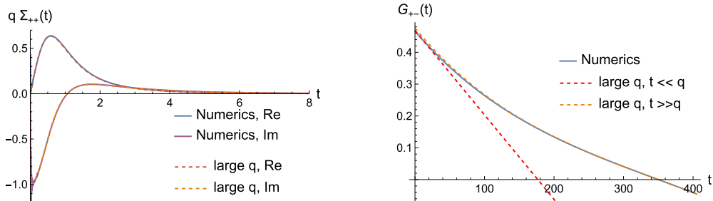
FIG. 5. Comparison between the large q complex solution and the numerical solutions ( q = 96 , \mathcal{J} = 1 , \hat{\mu} = 0.5 , T_L = 700 ). The vertical axis is q \Sigma_{++} \simeq \mathcal{J}^2 e^{g_{++}} for the left panel and G_{+-} for the right panel.
