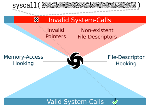
Fig. 2: By default, randomly-generated system-calls cannot reach deep kernel-code paths, as the arguments quickly trigger error conditions. FUZZNG’s hooks effectively “reshape” the input-space, transforming nonsensical pointer and file-descriptor arguments into valid ones, without introducing impossible behaviors. Through FUZZNG’s kernel hooks, system-calls that would normally result in trivial error conditions, produce interesting behaviors. In this figure and Figure 3, the “warp-hole” symbol represents the parts of FUZZNG that reshape the input-space.
