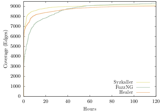
Fig. A3: Coverage comparison between Syzkaller and FUZZNG, while fuzzing KVM, over time. Syzkaller rapidly achieves high coverage over KVM, due to its extensive descriptions. However, eventually FUZZNG overtakes Syzkaller.
