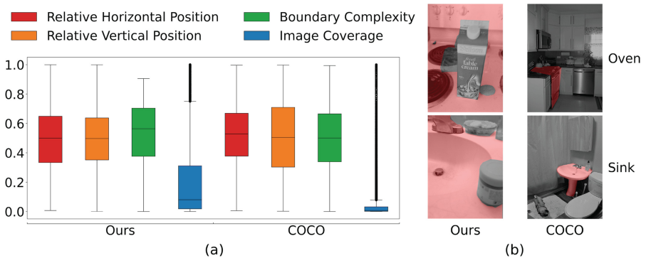
Fig. 2. Comparison of our dataset with the only existing few-shot instance segmentation dataset, COCO-20 i . (a) Summary statistics for all segmented objects in each dataset are shown in the box plot with respect to the location (i.e., relative x-coordinates and y-coordinates for mass center), boundary complexity, and image coverage. The box plot’s central mark denotes the median score, box edges the 25th and 75th percentiles scores, whiskers the most extreme data points not considered outliers, and individually plotted points the outliers. (b) Annotations from both datasets exemplify our quantitative finding that an object with larger image coverage is an outlier in COCO-20 i while common in our dataset.
