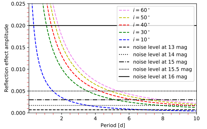
Fig. 15. Amplitude of the reflection effect of a typical sdB+DM system for different periods and inclinations. The black lines mark the TESS noise level for stars of different brightness.
