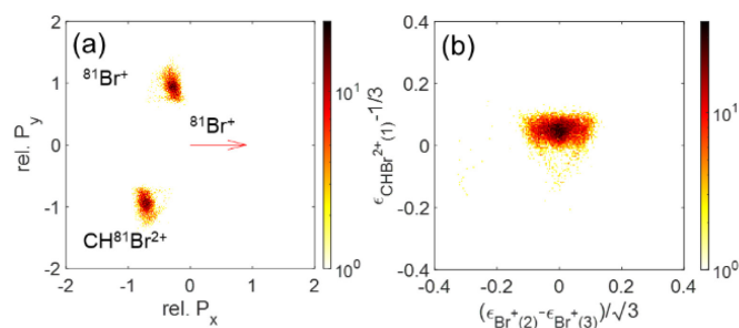
Fig. 13 Newton plots of the \text{Br}^+ + \text{Br}^+ + \text{CHBr}^{2+} channel with (a) \text{Br}^+ as reference fragment. (b) Dalitz plot for the same fragmentation channel.
