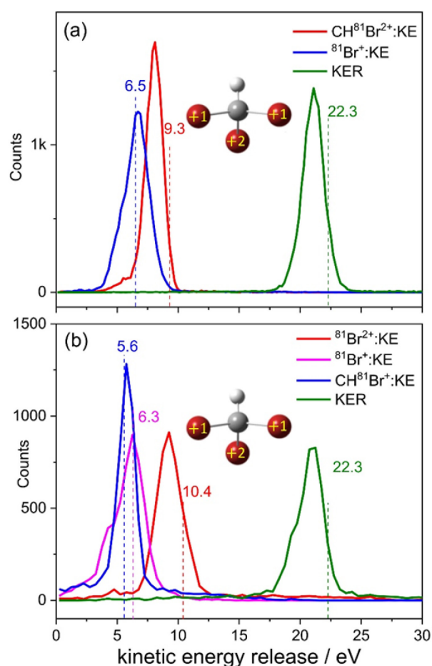
Fig. 12 Kinetic energy release distribution in three-body fragmentation of bromoform trication into (a) \text{Br}^+ + \text{Br}^+ + \text{CHBr}^{2+} and (b) \text{Br}^{2+} + \text{Br}^+ + \text{CHBr}^+ . The vertical dashed lines and numerical values are the results of our CES for concerted fragmentation with the charge distributions shown in the respective insets.
