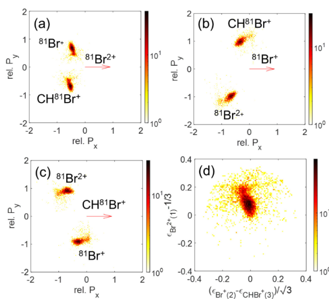
Fig. 14 Newton plots of the \text{Br}^{2+} + \text{Br}^+ + \text{CHBr}^+ channel with (a) \text{Br}^{2+} , (b) \text{Br}^+ , or (c) \text{CHBr}^+ as the reference fragment. (d) Dalitz plot for the same fragmentation channel.
