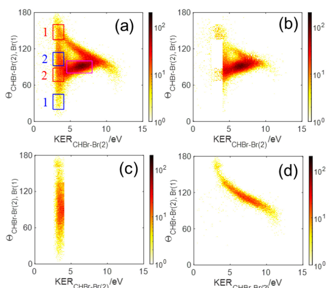
Fig. 6 Native frames analysis of the three-body fragmentation of bromoform trication into \text{Br}^+ + \text{Br}^+ + \text{CHBr}^+ assuming a \text{CHBr}_2^{2+} intermediate molecule: (a) All events, (b) after subtraction of sequential breakup via \text{Br}^+(1) + \text{CHBr-Br}^{2+}(2) and \text{Br}^+(2) + \text{CHBr-Br}^{2+}(1) , which are shown in panels (c) and (d), respectively. The red and blue rectangles shown in panel (a) mark the regions in which we replace the events within the regions marked in red by the equivalent events from the blue regions labeled with the same number to avoid contributions from other overlapping processes (see text). The magenta rectangle marks the region used to select concerted events.
