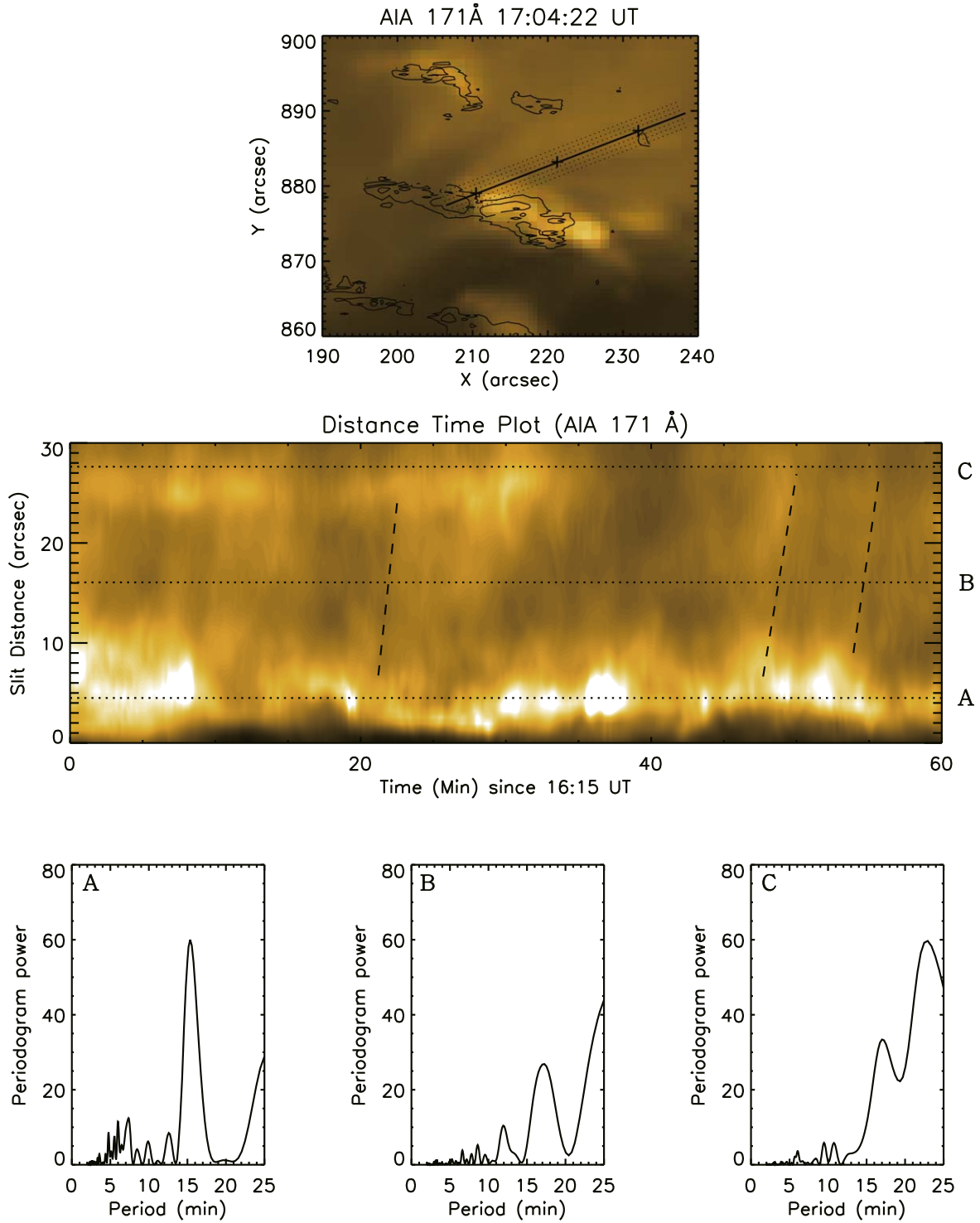
Figure 7. Top: AIA 171 Å intensity image with slit position along the plume. Contours indicate the brightness temperature. Middle: TD intensity plot along the slit in the top panel showing repetitive brightenings at the base of the plume and associated PDs. Horizontal and slanted dotted lines are used to archive typical power spectra and propagation speed of the PDs, respectively. Bottom: typical power spectra at the distance marked with the dotted lines in the middle panels.
