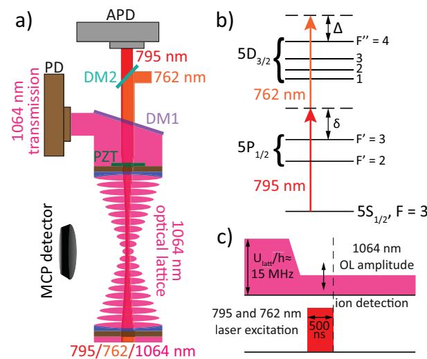
Figure 1. (Color online) Outline of experimental setup (a), utilized laser excitation scheme (not to scale) (b), and timing sequence of laser excitation and photoionization (c). “APD” avalanche photo-detector; “PD” photo-diode; “DM” dichroic mirror; “PZT” piezo-electric transducer. See text for details.
