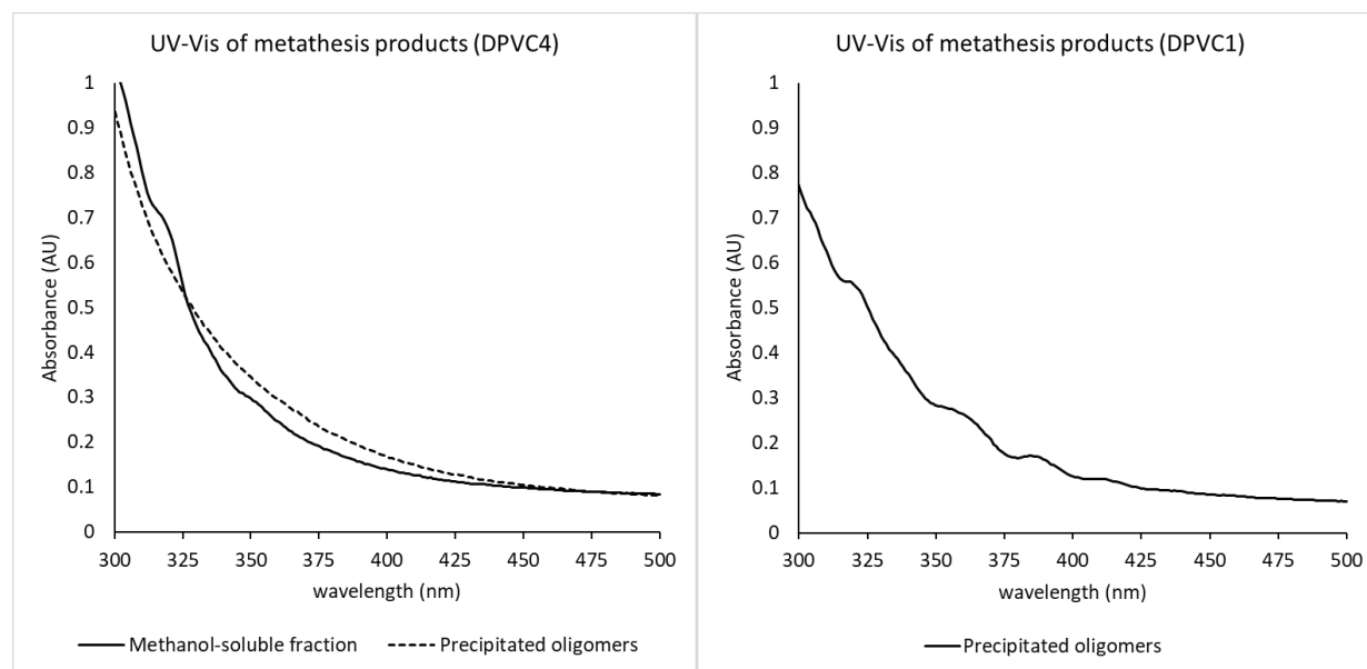
Figure 4: Left: UV-Vis of the metathesis products of DPVC4 (entry 4, Table 2). The fraction that precipitates in methanol is shown with a dotted line, and the remainder (recovered by evaporation of MeOH) with a solid line. Right: UV-Vis of the metathesis products of DPVC1 (entry 1, Table 2). The fraction that precipitates in methanol is shown. All UV-Vis spectra were taken in THF.
