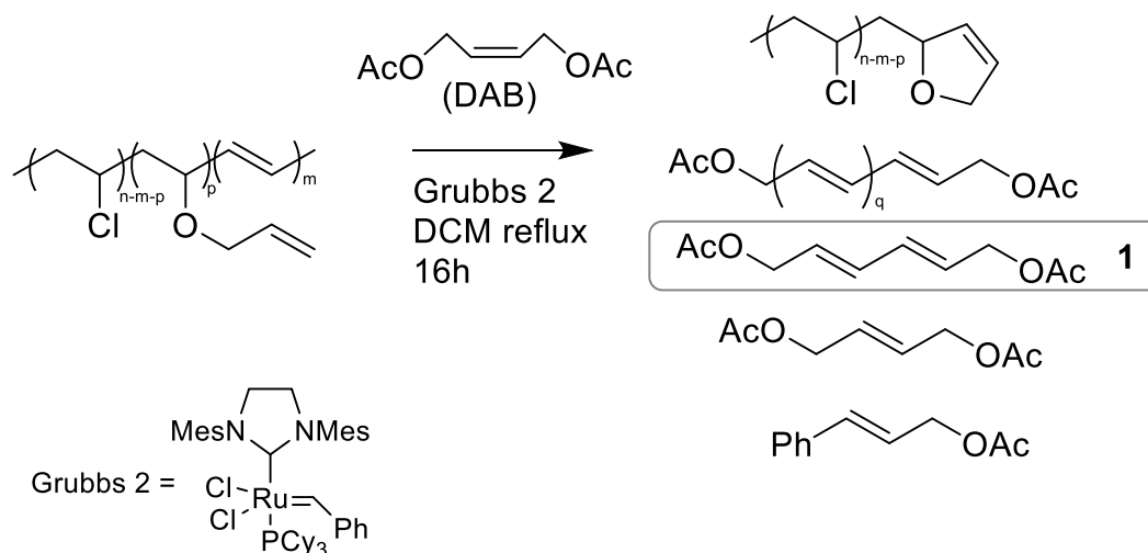
Scheme 4: Expected products from the metathesis reaction. Cinnamyl acetate is formed from the initial reaction of DAB with the Grubbs catalyst containing a Ph-CH= moiety. Trans -DAB is formed by self-metathesis of cis -DAB.
