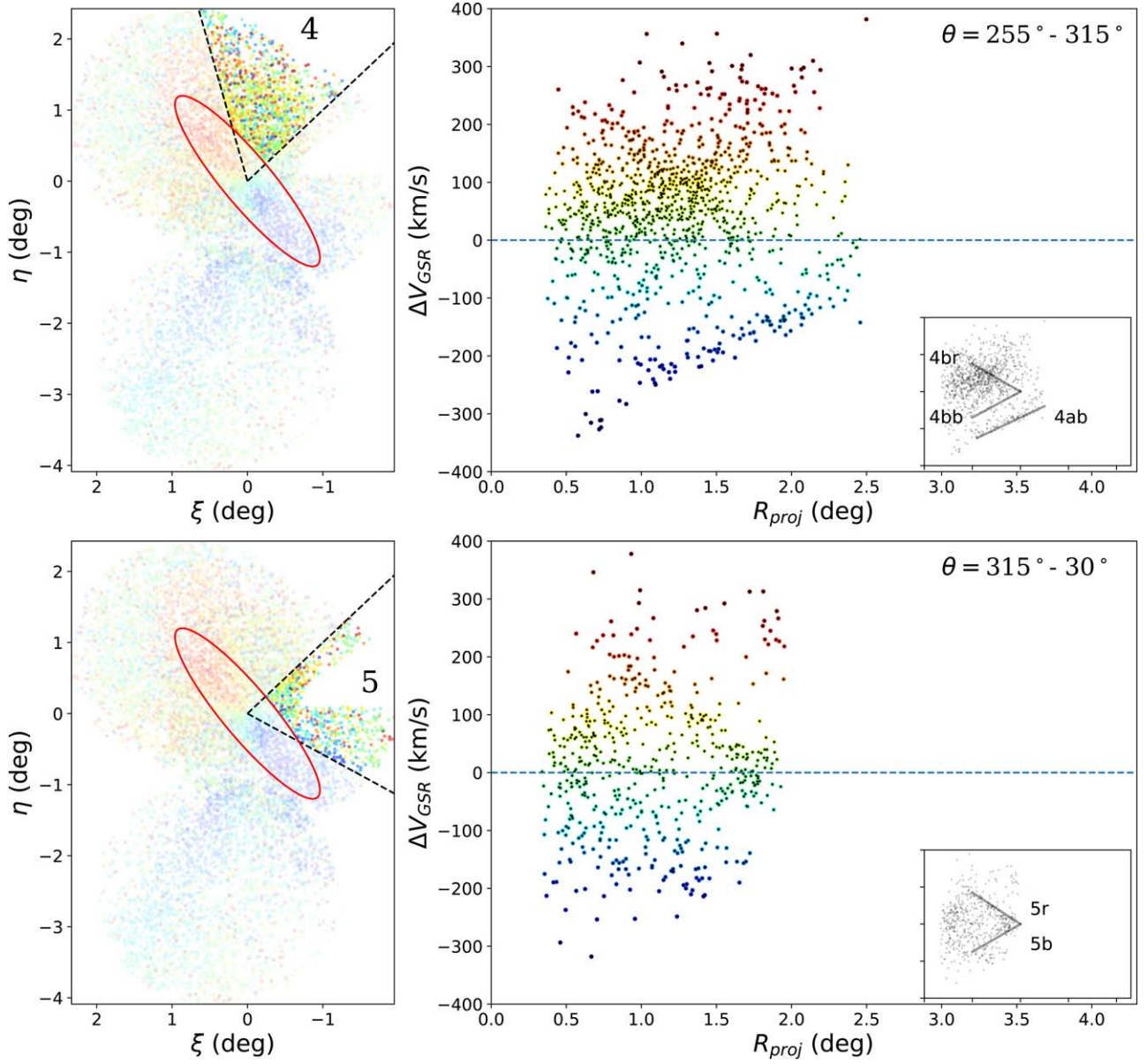
Figure 7. As in the previous figure, for two additional zones. Zone 5 includes the Western Shelf.
