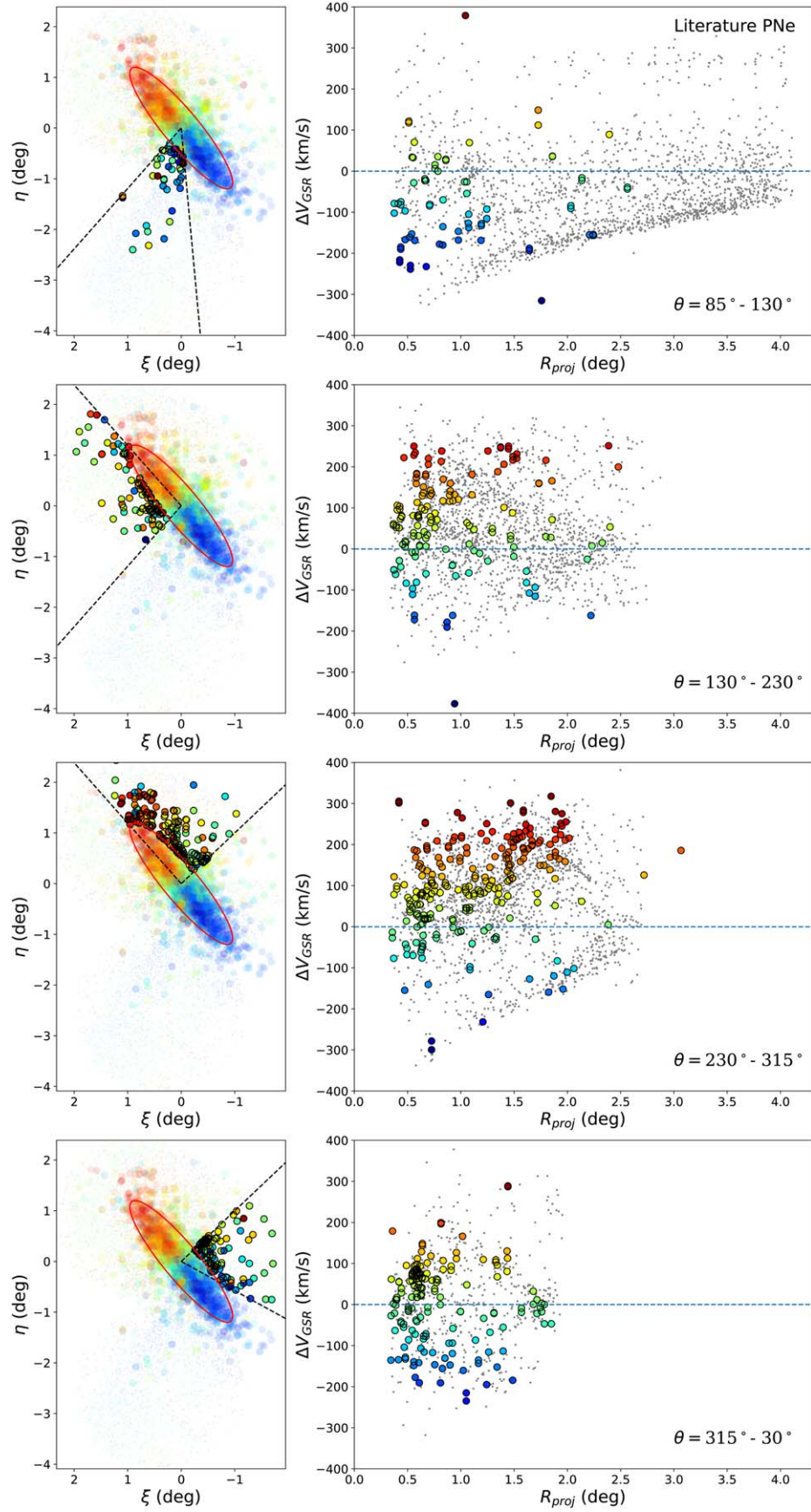
Figure 11. The distribution of known PNe from the literature (large colored circles; see the text) overlaid on M31 stars (smaller points).
