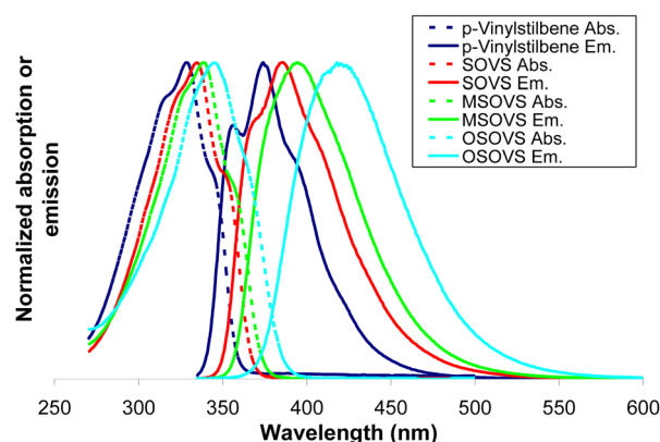
Fig. 16 UV-Vis and PL spectra of R -vinylstilbeneOS in THF [reproduced from ref. 110 with permission from American Chemical Society, 2008]. 110
