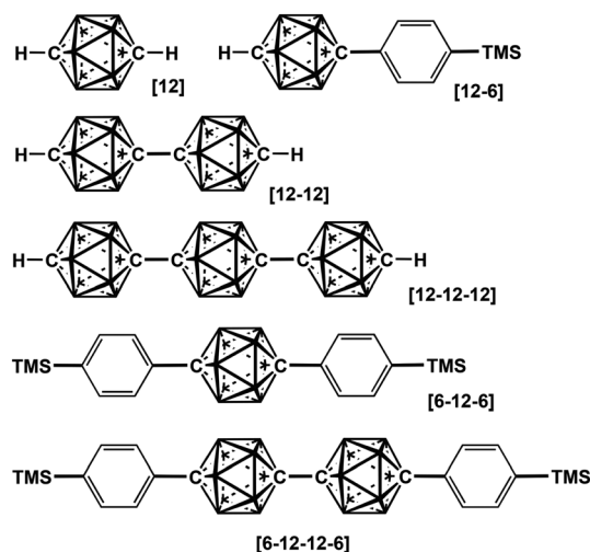
Fig. 2 Examples of carborane oligomers [reproduced from ref. 60 with permission from American Chemical Society, 2018]. 60
