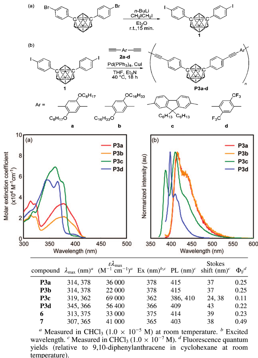
Fig. 4 Copolymers of bis( p -bromophenyl m -Carborane) with various p -aromatic dialkynes [reproduced from ref. 64 with permission from American Chemical Society, 2009]. 64
