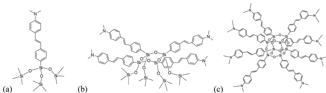
Fig. 18 (a) Me 2 NStil-corner, (b) Me 2 NStil-half, and (c) [Me 2 NStilSiO 1.5 ] 8 [reproduced from ref. 107 with permission from American Chemical Society, 2010]. 107
