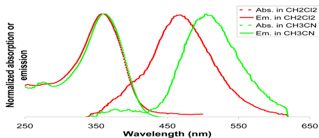
Fig. 17 UV-Vis and emission data for NSOVS in two good solvents [reproduced from ref. 111 with permission from American Chemical Society, 2008]. 111
