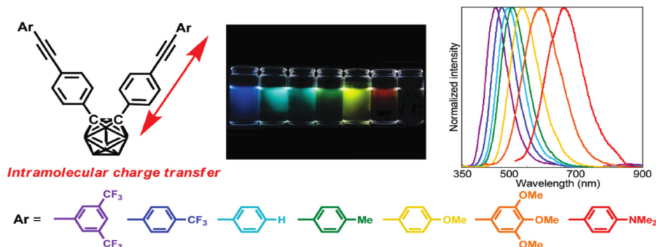
Fig. 3 Alkyne appended orthocarborane [reproduced from ref. 67 with permission from American Chemical Society, 2011]. 67
