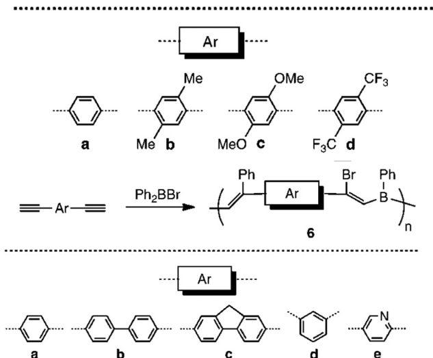
Fig. 5 General synthetic routes to alkenyl and bromoalkenyl polyboranes [reproduced from ref. 62 with permission from American Chemical Society, 2010]. 62
