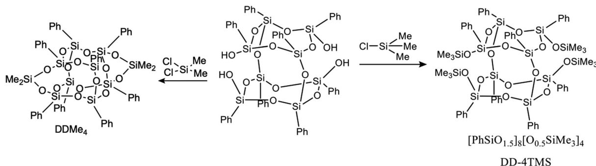
Fig. 28 Capping of commercially available tetrasilanol allows further functionalization [reproduced from ref. 117 with permission from American Chemical Society, 2019]. 117
