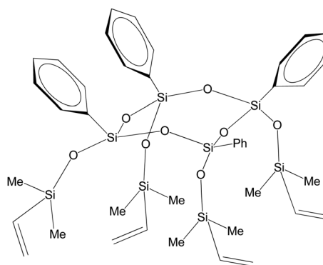
tetra(vinyl)dimethylsiloxane capped half cage
