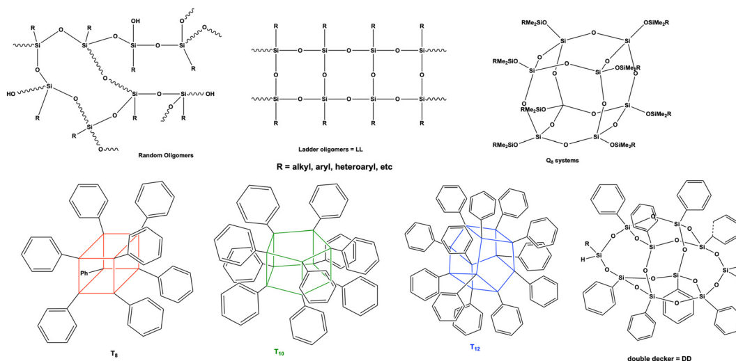
Fig. 10 Examples of various T ( \text{RSiO}_3 ) and Q ( \text{SiO}_4 ) cages.
