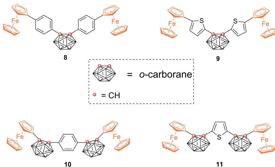
Fig. 6 Oligomers of o -carborane bonded to ferrocene and selected aromatic bridging systems [reproduced from ref. 68 with permission from Royal Chemical Society, 2020]. 68
