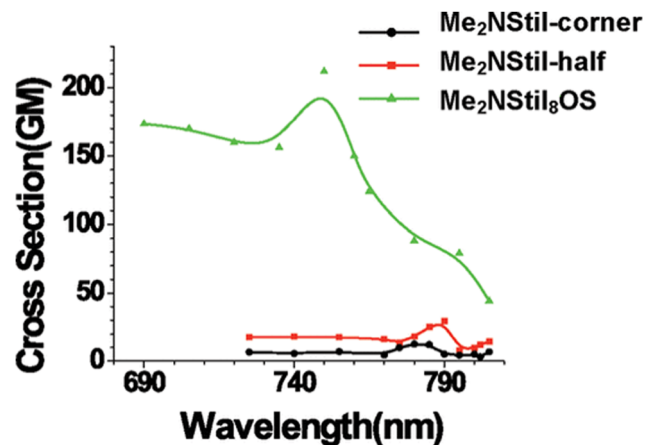
Fig. 19 Two-photon absorption cross-section spectra for the investigated chromophores [reproduced from ref. 107 with permission from American Chemical Society, 2010]. 107
