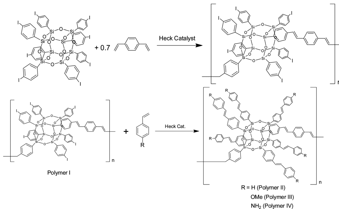
Fig. 24 Copolymerization of divinylbenzene with \text{I}_8\text{OPS} then further functionalization [reproduced from ref. 115 with permission from American Chemical Society, 2013]. 115
