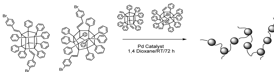
Fig. 22 Heck coupling vinyl 2 Ph x T 10 /T 12 SQs with BrSty 2 Ph x T 10 /T 12 SQs ( x = 8 and 10 ) [reproduced from ref. 112 with permission from American Chemical Society, 2010]. 112
