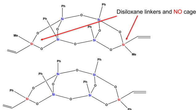
Fig. 37 Vinyl-disiloxane capped ladder (LL) silsesquioxane [reproduced from ref. 126 with permission from American Chemical Society, 2019]. 126
