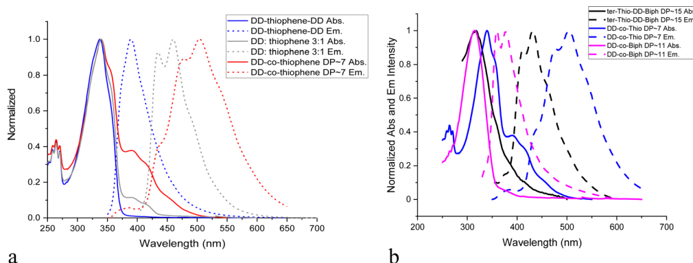
Fig. 36 (a) Normalized absorption and emission of DD-thiophene-DD, mixture of DD:thiophene 3:1 and longer DD-co-thiophene (1:1). (b) Absorption and emission of ter-thio-DD-biph and corresponding copolymers, DD-co-biphenyl and DD-co-thiophene. 125
