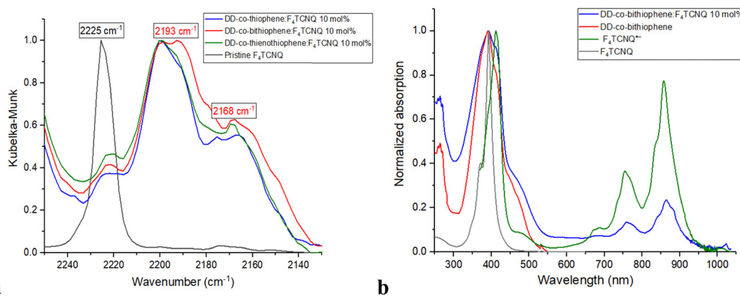
Fig. 34 (a) The characteristic region of \nu\text{C}\equiv\text{N} in FTIR spectra for DD-co-thiophene, -bithiophene, -thienothiophene mixing with 10 mol% \text{F}_4\text{TCNQ} and pristine \text{F}_4\text{TCNQ} [reproduced from ref. 122 with permission from Wiley, 2021]. 122
