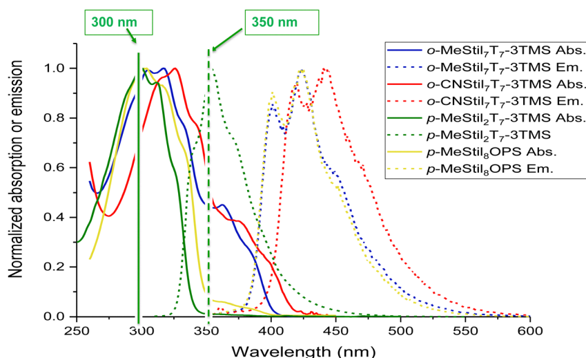
Fig. 29 Photophysical characterization of corner missing phenyl cage [reproduced from ref. 116 with permission from American Chemical Society, 2019]. 116
