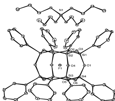
Fig. 14 OPS with an encapsulated F - [reproduced from ref. 108 with permission from Wiley, 2003]. 108
