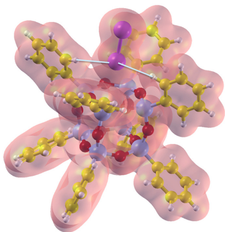
Fig. 12 \text{Br}_2 absorption centrally above the \text{T}_8 cage face is preferred. The face has two phenyls oriented with hydrogens in (wing) and two turned at 90^\circ . \text{Br}_2 is stabilized in this configuration by hydrogen bonding to the closer Br atom and the two o -hydrogens on the wing-oriented phenyls. Polarization occurs coincidentally as the \text{Br}_2 interacts with the \text{T}_8 face [reproduced from ref. 103 with permission from Royal Chemical Society, 2014]. 103
