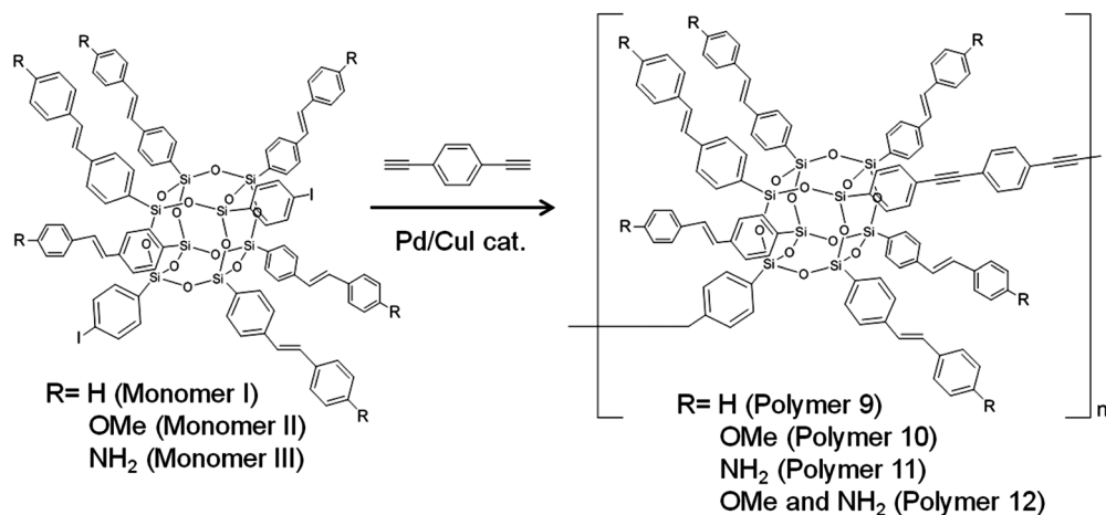
Fig. 25 Syntheses of dialkynyl copolymers [reproduced from ref. 115 with permission from American Chemical Society, 2013]. 115
