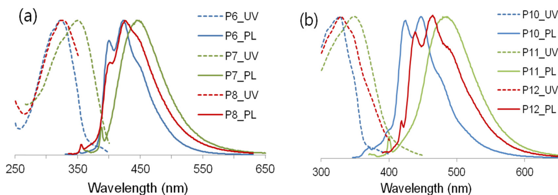
Fig. 26 UV-vis and emission spectra for methoxystilbene polymers, aminostilbene polymers and their terpolymers in THF [reproduced from ref. 114 with permission from American Chemical Society, 2013]. 114
