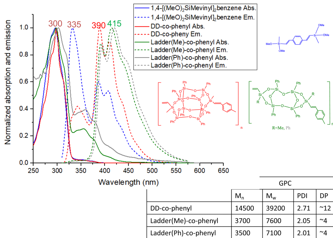
Fig. 38 UV/vis spectra of DD-co-phenyl, LL-co-phenyl and model compound [reproduced from ref. 122 with permission from Wiley, 2021]. 122
