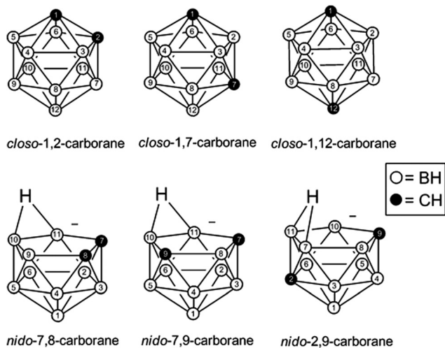
Fig. 1 Examples of well-known carborane structures [reproduced from ref. 63 with permission from American Chemical Society, 2011]. 63
