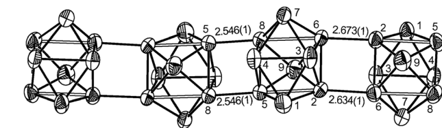
Fig. 7 (Rb-18C6)_8[Ge_9=Ge_9=Ge_9=Ge_9] 2en 18C6 is crown ether and en is ethylene diamine [reproduced from ref. 69 with permission from American Chemical Society, 2003]. 69
