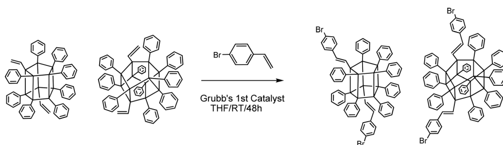
Fig. 21 Alkene metathesis of vinyl 2 Ph x ( x = 8 and 10 ) T 10 and T 12 SQs with 4-bromostyrene [reproduced from ref. 112 with permission from American Chemical Society, 2010]. 112
