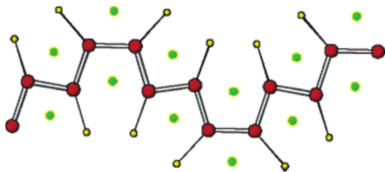
Fig. 9 Fragment of flat zigzag chain in \text{LiMg}(\text{Eu}/\text{Sr})_2\text{Sn}_3 with coplanar Li/Mg mixed occupancy positions (M), resembling a polyacetylene, (\text{CH})_\infty . Chain. \text{Eu}/\text{Sr} = light-green spheres above and below plane of chain [reproduced from ref. 70 with permission from American Chemical Society, 2005]. 70
