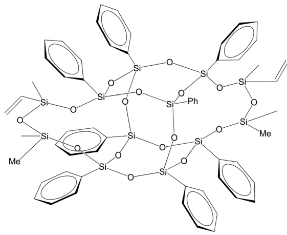
tetra(vinylmethyl)disiloxane capped DD, Viny14XDD
