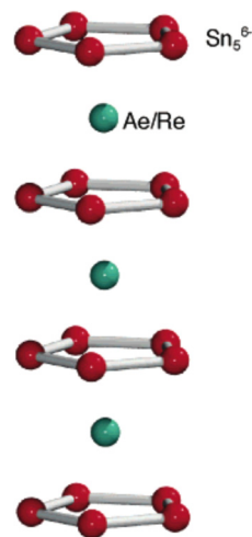
Fig. 8 Stacked Sn_5^{6-} aromatic rings separated by Ca/Eu (AeRe) cations [reproduced from ref. 70 with permission from American Chemical Society, 2005]. 70
