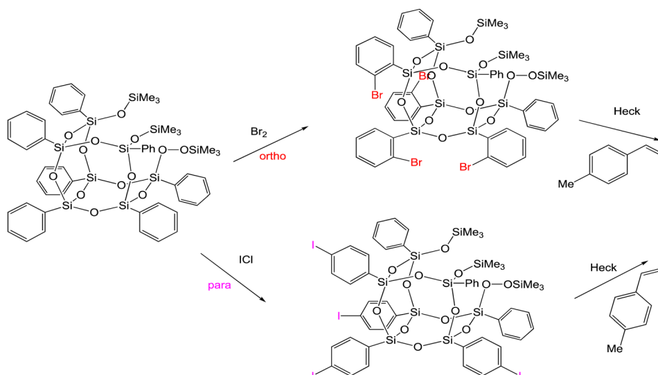
Fig. 27 Capping of commercially available trisilanol allows further functionalization. 116
