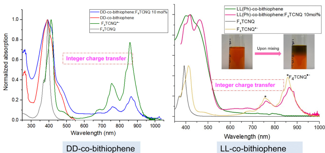
Fig. 40 Solution mixing of F 4 TCNQ CT with DD-co-bithiophene and LL-co-bithiophene revealing integer charge transfer [reproduced from ref. 122 with permission from Wiley, 2021]. 122
