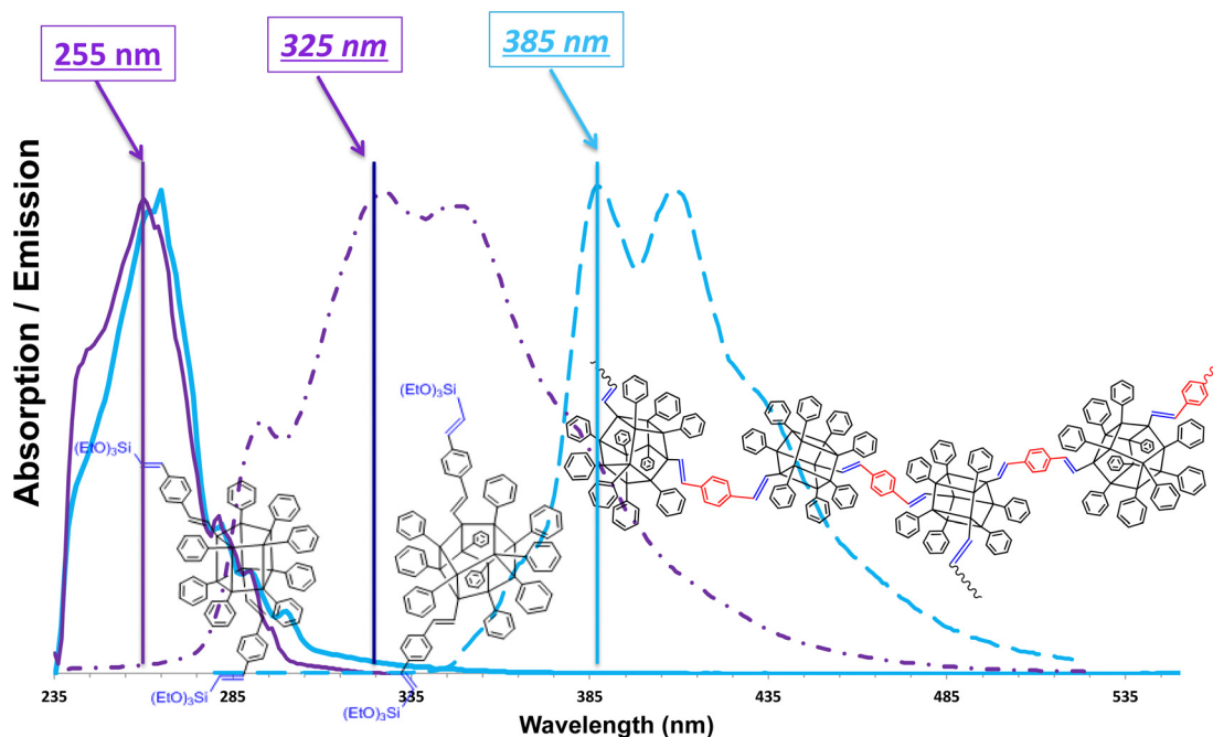
Fig. 23 Solution absorption and emission spectra (THF, \lambda_{\text{excitation}} = 265 \text{ nm} ) of "beads on a chain" and the corresponding model -\text{Si}(\text{OEt})_3 compounds [reproduced from ref. 112 with permission from American Chemical Society, 2010]. 112
