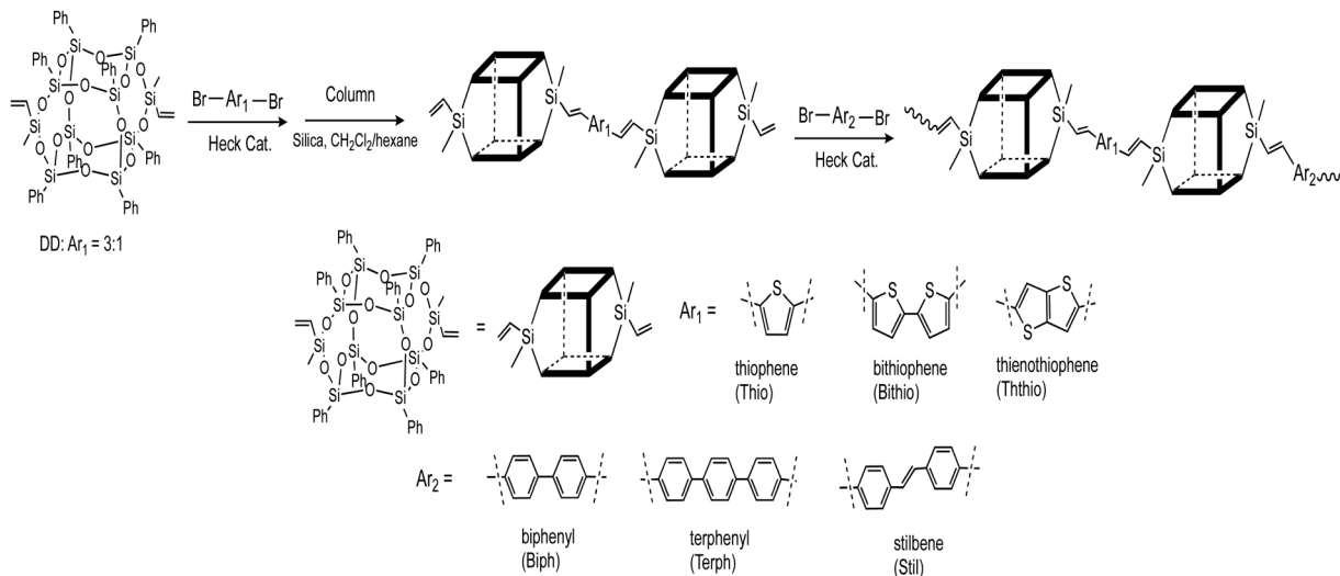
Fig. 35 General approach to synthesizing DD based alternating terpolymers. 125
