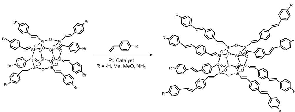
Fig. 15 R = -H (SOVS), ( p -Me) MSOVS, p -MeO (OSOVS, p -NH 2 (NSOVS) [reproduced from ref. 110 with permission from American Chemical Society, 2008]. 110
