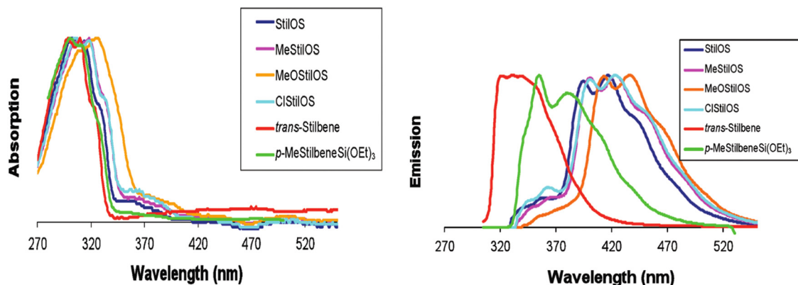
Fig. 13 (a) Normalized absorption. (b) Emission of [( p -4- R -stilbene)SiO 1.5 ] 8 in THF [reproduced from ref. 107 with permission from American Chemical Society, 2010]. 107
