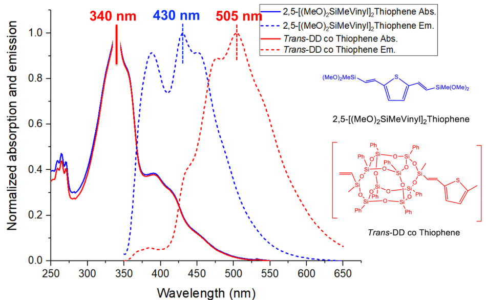
Fig. 33 Photophysics of [vinylDDvinyl-thiophene] x where x > 20 .
