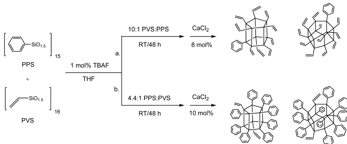
Fig. 20 Fluoride-mediated rearrangement of PPS and PVS to (a) vinyl x Ph 1 ( x = 9 and 11 ) T 10 and T 12 and (b) vinyl 2 Ph x ( x = 8 and 10 ) T 10 and T 12 silsesquioxanes [reproduced from ref. 112 with permission from American Chemical Society, 2010]. 112
