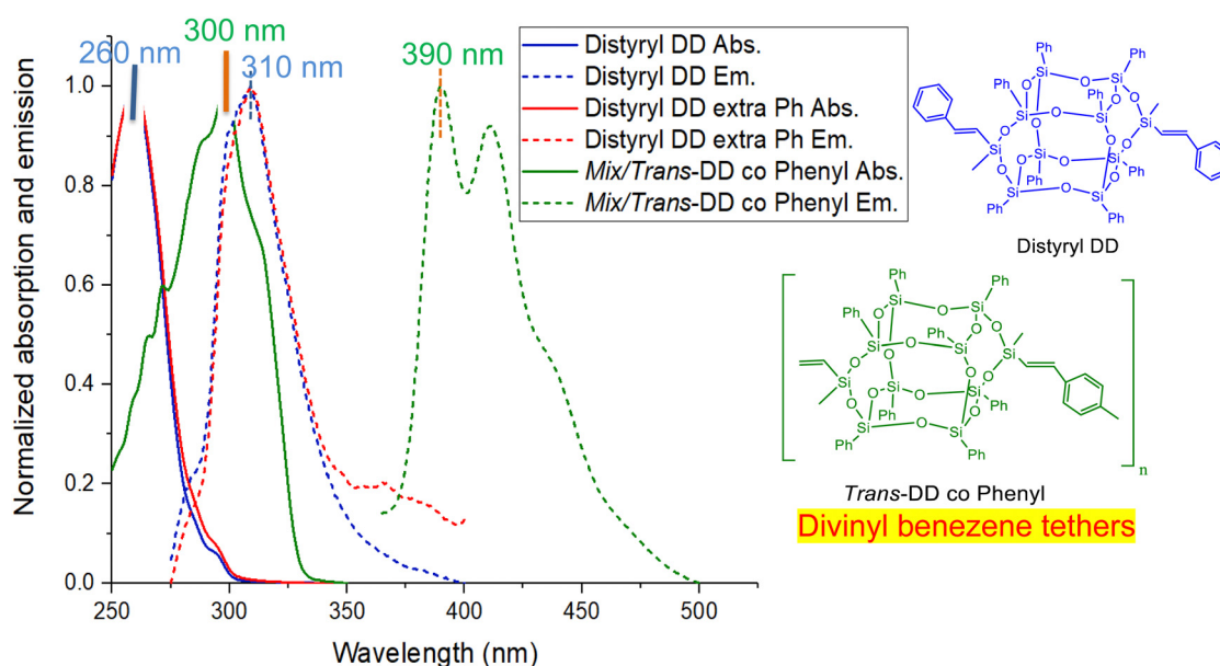
Fig. 32 Photophysics of [vinylDDvinyl-Ph] x where x > 20 .
