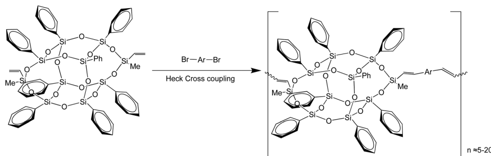
Fig. 31 Copolymerization of vinyl 2 DD with dibromoaromatic compounds [reproduced from ref. 117 with permission from American Chemical Society, 2019]. 117
