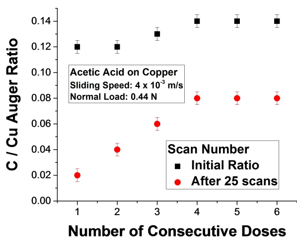
Figure 4. Plot of the initial (■) and final (●) C(KLL)/Cu(LMM) Auger ratios after 25 rubbing cycles for repeated dosing of the surface without cleaning the sample between doses. Experiments were performed at a load of 0.44 N and a sliding speed of 4 \times 10^{-3} m/s. Reprinted with permission from Ref. [1], Copyright 2021 Springer.
