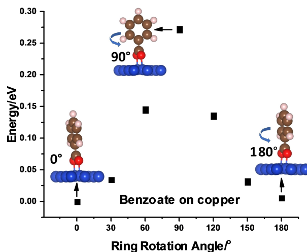
Figure 10. Energy variation for benzoate species on a Cu(100) slab obtained by using density functional theory as a function of azimuthal rotation angle of the aryl ring with respect to the adsorbed acetate species. Shown on the figure are depictions of how the structure varies with rotation angle.
