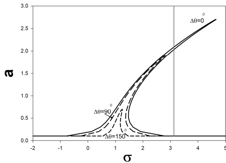
Figure 4. Schematic illustration of the amplitude-frequency response of the forced array of coupled waveguides due to self-interaction. The frequency \sigma = \frac{1}{\varepsilon}(2\omega_2 - \omega_1 - \omega_{0,n}) is normalized to \delta\Gamma_1 . For illustrative purposes, we have taken \frac{3\delta}{8\omega_{0,n}} = 0.5 , (\delta\Gamma_2)^2 = 0.008 , and \mu^2 = 0.00425 . We consider three values for \Delta\theta = 0, 90, 150^\circ .
