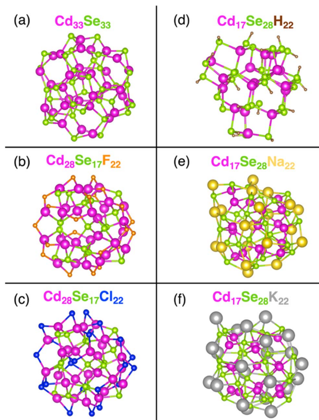
Fig. 1 The DFT optimized geometry of stoichiometric (a) \text{Cd}_{33}\text{Se}_{33} , and non-stoichiometric: Cd-rich (b) \text{Cd}_{28}\text{Se}_{17}\text{F}_{22} , (c) \text{Cd}_{28}\text{Se}_{17}\text{Cl}_{22} and Se-rich (d) \text{Cd}_{17}\text{Se}_{28}\text{H}_{22} , (e) \text{Cd}_{17}\text{Se}_{28}\text{Na}_{22} , (f) \text{Cd}_{17}\text{Se}_{28}\text{K}_{22} quantum dots (QDs). Anionic ligands bond to the surface Cd atoms and cationic ligands bind to the surface Se atoms. Each \text{H}^+ is monodentate i.e. , it coordinates only one Se atom per ligand and leads to the formation of a polar covalent \text{H}-\text{Se} bond. The denticity of other ligands ranges from two in Cd-rich QDs to two to four in Se-rich QDs, due to the more ionic interaction.
