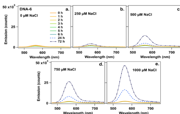
Figure 3 Emission spectra for DNA-6 at 0 to 6, 24, and 72 h (legend) without NaCl (0 μM) and after addition of NaCl at b) 250 μM, c) 500 μM, d) 750 μM, and e) 1000 μM.
