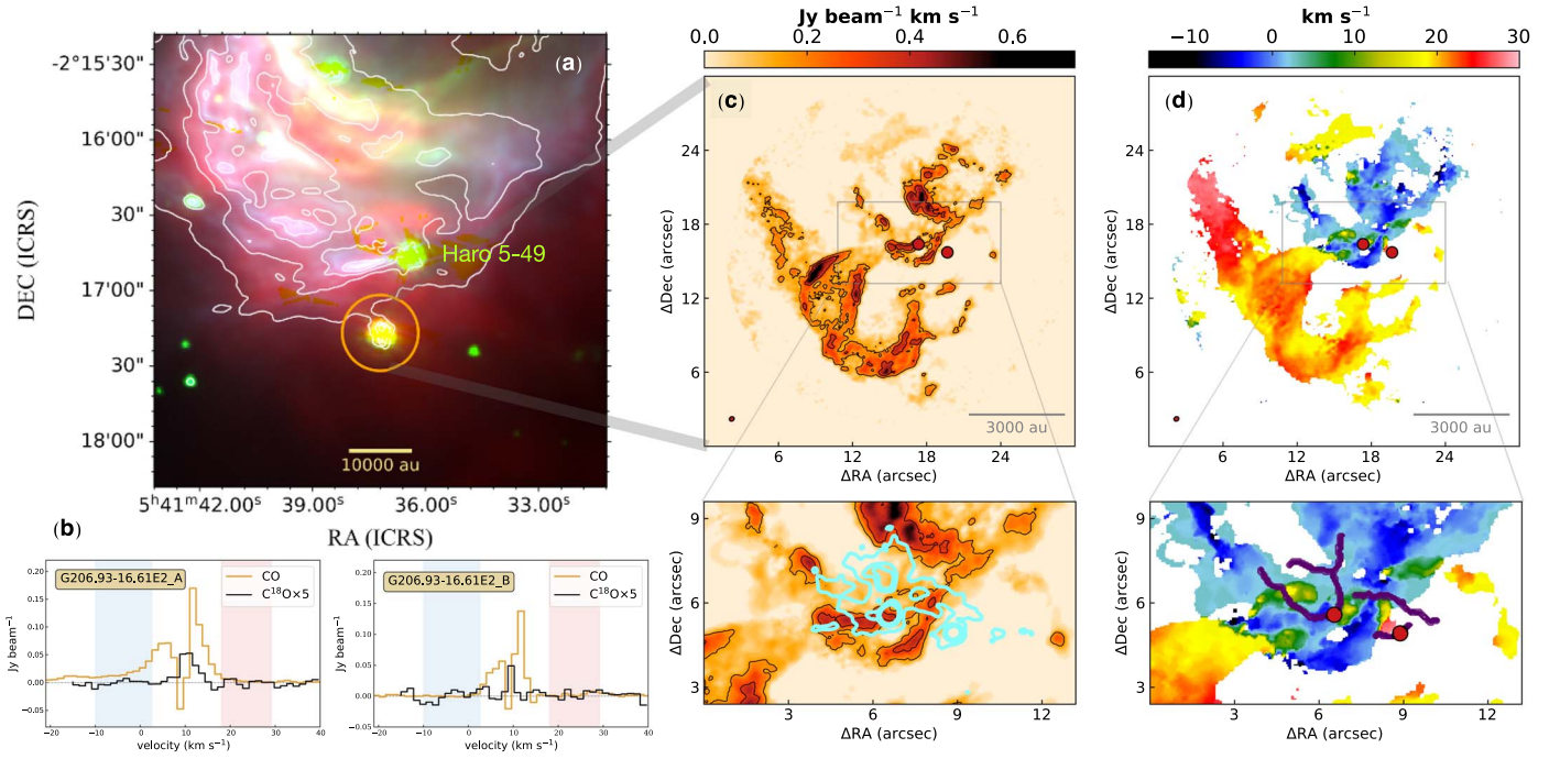
Figure 2. The CO outflow from G206.93-16.61E2. (a) The color image is the same as in Figure 1(a). The white contours show the Spitzer 8\ \mu\text{m} emission. The orange circle shows the FOV of the ALMA image. (b) \text{C}^{18}\text{O} and ^{12}\text{CO}\ J=2-1 spectra at the positions of G206.93-16.61E2_A and G206.93-16.61E2_B. The blue and red shaded areas define the blue- and redshifted high-velocity emission of the ^{12}\text{CO} line emission. (c) Moment 0 map of all high-velocity emission combined ( [-10\ \text{to}\ 2.6]\ \text{km}\ \text{s}^{-1} for blue and [18\ \text{to}\ 29.2]\ \text{km}\ \text{s}^{-1} for red), as defined in panel (b), with contours of 10\sigma_{\text{out}} and 25\sigma_{\text{out}} ( 1\sigma_{\text{out}} = 33\ \text{mJy beam}^{-1} ). The zoom-in picture shows the same image, with dust continuum contours in cyan at 3\sigma_{1.3\ \text{mm}} , 10\sigma_{1.3\ \text{mm}} , and 20\sigma_{1.3\ \text{mm}} . (d) Moment 1 map of high-velocity emission. The red circles represent the protostars E2_A and E2_B. The structures of the continuum ribbons identified by Filfinder are shown with purple lines.
