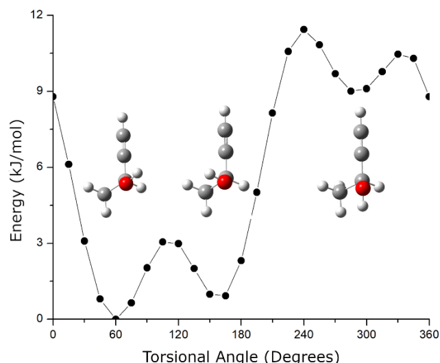
Figure 2 The conformational potential energy surface (PES) for butynol is shown. The relaxed PES is calculated using the B3LYP GD3BJ 6-311++G(d,p) model chemistry. The structures for the three stable conformers are also shown.
