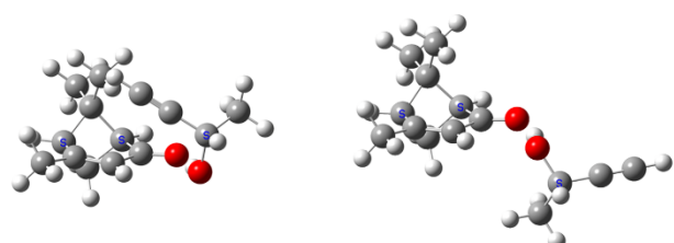
Figure 1 The structural characterization of the lowest energy isomers of the 1:1 complexes formed between verbenone and butynol is illustrated. The two hydrogen bond positions are shown in the top panel (A). Most quantum chemistry methods identify two equilibrium geometries for the dihedral angle around the O---O axis of the hydrogen bond as shown in panel (B). The structures shown in this figure are equilibrium geometries from the B3LYP GD3BJ def2TZVP calculation set.
