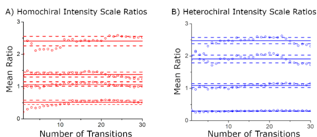
Figure 5 This figure illustrates the scaling process used to determine the isomer composition of the homochiral and heterochiral sets of isomers. Each data point gives the average scale factor between the experimental transition intensities and a simulated spectrum using experimental rotational constants (and distortion constants) and theoretical dipole moment components after the N strongest transitions have been analyzed. The solid horizontal lines are the average scale factor and the dotted lines are 1 standard deviation limits.
