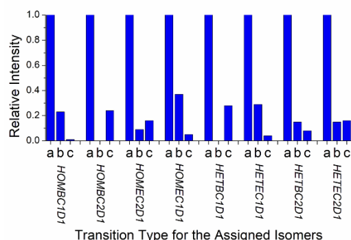
Figure 11 The top panel shows the experimental determination of the relative intensities of the a-, b-, and c-type rotational spectrum components for the 8 chiral tag complexes identified in this work. These relative intensities are governed by the ratio of the squares of the a-, b-, and c-components of the dipole moment vector represented in the principal axis system. The relative intensities of the square of the dipole moment components in the B3LYP GD3BJ def2TZVP calculations are shown in the bottom panel.
