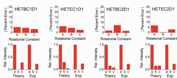
Figure 12 This figure illustrates the way that the spectral assignments guided by quantum chemistry are used to establish the absolute configuration of verbenone. Panel (A) shows the comparison between the experimental spectrum parameters for the highest abundance species observed when (S)-butynol is used as the tag and the lowest energy isomers of homochiral and heterochiral complexes identified in the quantum chemistry analysis using B3LYP GD3BJ def2TZVP. This comparison uses the percent error for the rotational constants and a comparison of the relative spectral intensities to the square of the dipole moment components. The best match for the spectrum is to the homochiral complex, HOMBC1D1 – outlined in green. Since the spectrum matches a homochiral geometry and the tag is known to be (S)-butynol, the absolute configuration is established as (S)-verbenone. The confidence in this determination is increased by the fact that the other three spectra observed in the (S)-butynol tag measurement also have exclusive matches to theoretical homochiral geometries. Furthermore, the other four spectra, which dominate when (R)-butynol is the tag, exclusively match the theoretical heterochiral geometries – as shown in the supporting information.
