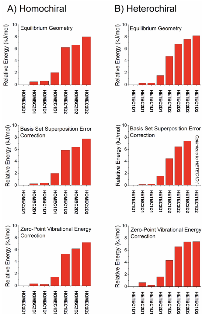
Figure 7 The relative isomer energies from calculations with the B3LYP GD3BJ def2TZVP model chemistry are shown with three different levels of approximation. The top set of results uses the equilibrium energies. The middle panel includes a counterpoise correction to account for basis set superposition error. The bottom panel uses equilibrium energies correct by the zero-point vibrational energy contribution using the harmonic approximation.
