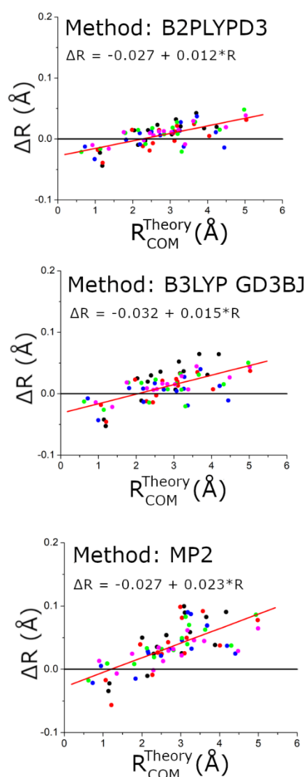
Figure 10 This figure shows the differences in the experimental and theoretical distance of each carbon atom from the center-of-mass of the chiral tag complex. The red line shows a linear regression analysis for each data set to help quantify the way these errors vary with the center-of-mass distance. The linear fit formulas are shown as insets in each figure. The coordinates come from the 5 structures that were measured with ^{13}\text{C} -sensitivity: HOMECD1 (black), HOMBC2D1 (blue), HOMBC1D1 (magenta), HETEC1D1 (red), and HETBC1D1 (green). The figure for calculations with the 6-311++G(d,p) basis set is shown in the supporting information.
