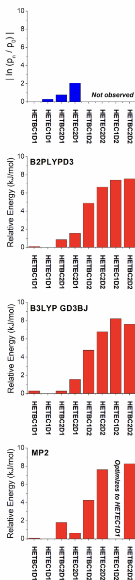
Figure 6 A graphical representation of the relative isomer energies reported in Table 1 for calculations with the def2TZVP basis set is shown. The three quantum chemistry methods are B2PPLYPD3, B3LYP GD3BJ, and MP2. In some cases, the geometry optimization collapsed into the lower energy geometry with different dihedral angle about the O---O axis of the hydrogen bond and these cases are indicated in the figure. An analogous figure using the 6-311++G(d,p) basis set is available in the supporting information.
