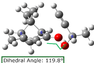
B) DFT without Dispersion Correction
