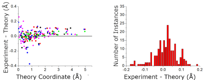
Figure 9 The accuracy of the quantum chemistry structures is benchmarked using the carbon atom coordinates – in the principal axis system for molecular rotation – obtained from the Kraitchman analysis. The scatter plot shows the difference in the absolute values of these coordinates (coordinate signs are unavailable from the spectroscopic analysis) as a function of the size of the coordinate. The coordinates come from the 5 structures that were measured with ^{13}\text{C} -sensitivity: HOMEC2D1 (black), HOMBC2D1 (blue), HOMBC1D1 (magenta), HETEC1D1 (red), and HETBC1D1 (green). The figure for calculations with the 6-311++G(d,p) basis set is shown in the supporting information.
