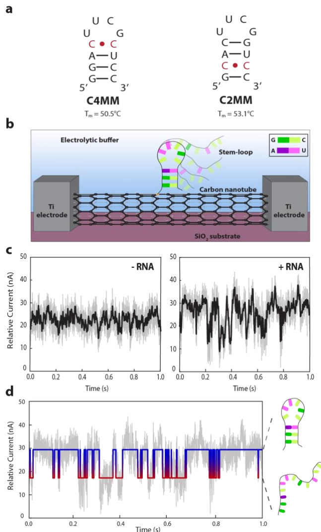
Figure 1. smFET experimental setup. (a) The two stem-loop constructs studied here each introduce a single mismatched base-pair within the stem of the stem-loop by substituting a cytosine for a guanine. (b) A schematic cartoon of the smFET experimental platform is shown. Each smFET device consists of a SWCNT that serves as a conductive channel between a source- and drain electrode, with a stem-loop construct tethered to the surface of the SWCNT. Details of device fabrication and characterization are described in the Supporting Information and Figure S1. (c) A representative, 1 s current versus time trajectory recorded before (left) and after (right) stem-loop tethering. The black line overlaid on the raw trajectory (light gray) is a 100 data point rolling average of the raw trajectory for visualization purposes. A quantitative analysis of these data demonstrating our ability to distinguish stem-loop-dependent transitions from smFET device noise are provided in Figure S2. (d) An idealized current state versus time trajectory (blue and red), obtained by applying a previously described two-state, drift-corrected, thresholding algorithm 35-36, 42 is overlaid on the current versus time trajectory. Details of the data analysis
