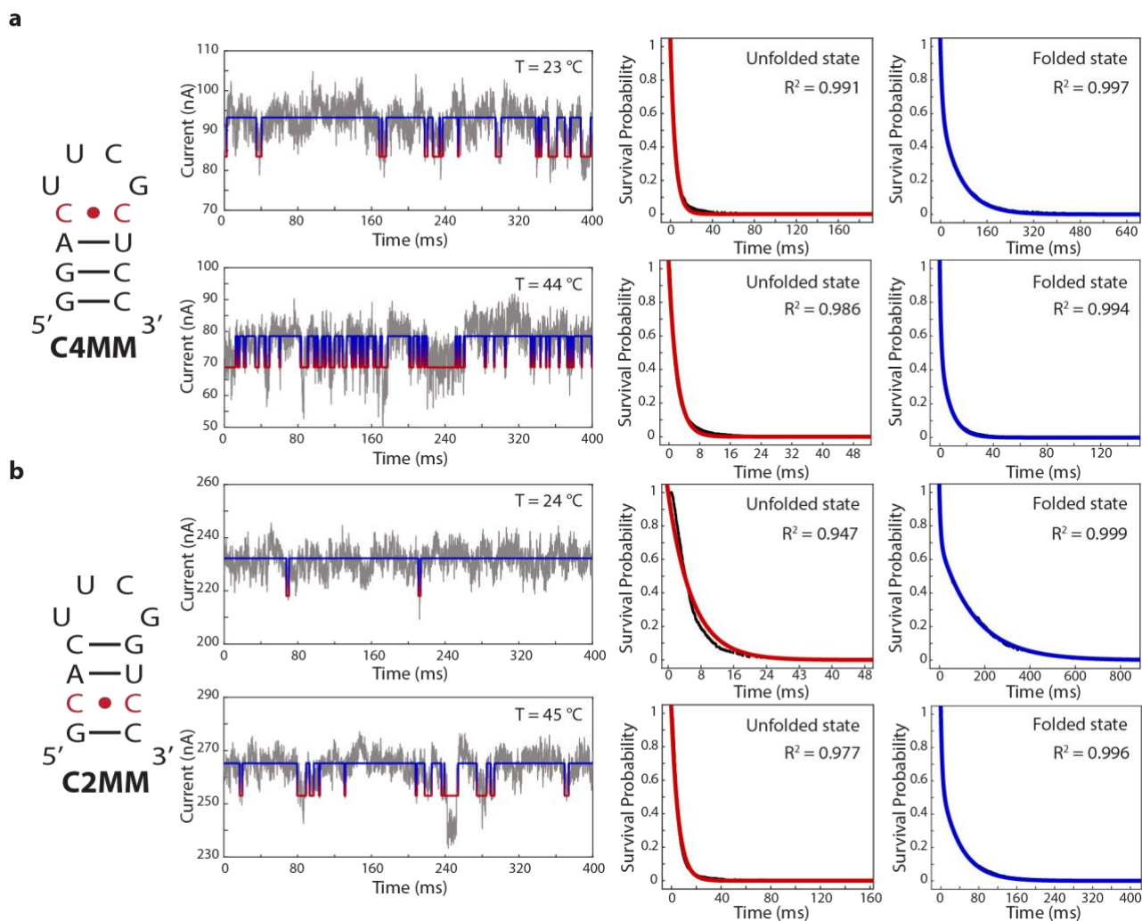
Figure 4. Kinetic analyses of C4MM and C2MM current versus time trajectories. Secondary structure diagrams of the stem-loop constructs with the mismatched base-pairs denoted in red (first column), representative current versus time trajectories (gray) with overlaid idealized current state versus time trajectories (blue and red) (second column), single-exponential fits (red curves) to the survival probability plots of the ensemble of unfolded conformations (black data points) at T_{\text{low}} (third column, top) and T_{\text{high}} (third column, bottom), and double-exponential fits (blue curves) to the survival probability plots of the ensemble of folded conformations (black data points) at T_{\text{low}} (fourth column, top) and T_{\text{high}} (fourth column, bottom) for (a) C4MM and (b) C2MM.
