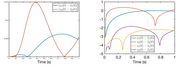
Fig. 4: The left figure presents the absolute point-wise error between the 161 st trajectory created by using the dynamics of the Duffing oscillator and the 161 st trajectory created by using the model described in (13). This figure also presents how the absolute point-wise error is progressing in time. Each curve in this figure represents a different state dimension. The figure on the right presents a comparison between the log absolute point-wise error for the 161 st trajectory when using OKDMD and the log absolute error for the 161 st trajectory when using POKeDMD. The figure also presents how the log absolute point-wise error is progressing in time. The OKDMD algorithm is the prior method that was used in [6] and it does not use the known portion of the dynamics in order to produce a model.
