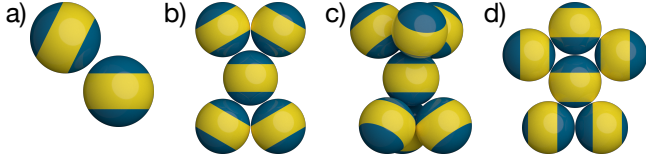
Fig. 1 (a) Triblock Janus spheres interacting via the Kern-Frenkel potential. Particles within the range of interaction ( \sigma < |\mathbf{r}_{ij}| \leq \lambda \sigma ) interact only if the patches are facing each other (i.e., if the vector joining the center of the particles intersects both patches, as in a). (b-c) Kagome and pyrochlore motifs formed by triblock Janus spheres with symmetric patches in 2D and 3D, respectively. (d) The snub square motif, which contains an asymmetric valence around each particle, suggesting a need for patches of unequal size.
