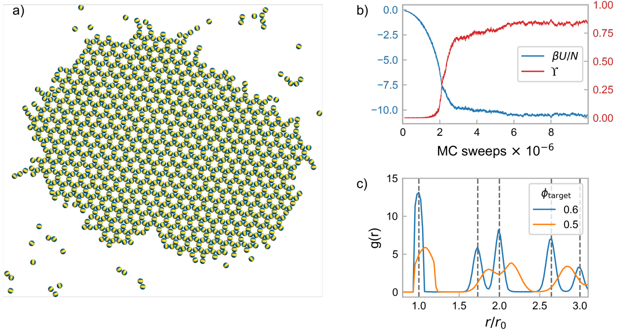
Fig. 3 Self-assembly results for the kagome lattice with \alpha^* = (37^\circ, 1.12, 5.8) obtained from alchemical simulations at b_2^0 = -4 and \phi_{\text{target}} = 0.60 (Figure 2a). (a) Snapshot of the last simulation frame showing the self-assembled kagome lattice. (b) Progression of the intensive potential energy \beta U/N and crystal yield \gamma (see Model and Methods). (c) RDFs of the assembled kagome structures for (b_2^0, \phi_{\text{target}}) = (-4, 0.6) and (-9, 0.5) ; the vertical dashed lines represent the RDF of the ideal kagome lattice. In all cases, the radial axis is normalized by the location of the first peak of the assembled structure at \phi_{\text{target}} = 0.6 , given by r_0 \approx 1.056 . The relative locations of the peaks in the assembled structure is in very good agreement with those of the ideal crystal. The RDFs were computed over the final 2 \times 10^6 MC sweeps of the assembly simulations.
