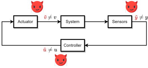
Figure 1: CPS block diagram and model of the adversaries considered in the paper. Variables highlighted in black are the uncompromised variable, while the red variables are the values the attacker might compromise.
