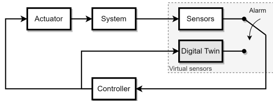
Figure 2: Virtual sensors.
