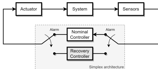
Figure 3: Simplex architecture.
