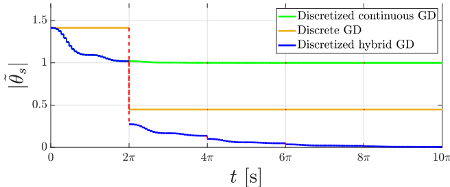
Fig. 1: The projection onto t of the norm of the estimation error \tilde{\theta}_s given sampled data, simulated using the HyEQ Toolbox [11].
