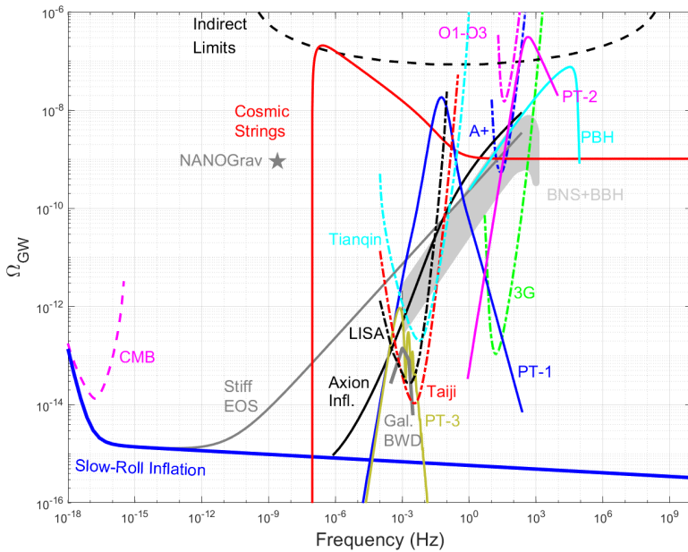
Fig. 1 Landscape of gravitational wave cosmology. Experimental results include: O1-O3 LIGO-Virgo upper limits [19], indirect limits from big bang nucleosynthesis [20], CMB limits [20], and NANOGraV pulsar timing measurement [21], as well as projected sensitivities of the third generation (3G) terrestrial GW detectors [22, 23] and space-borne LISA [24], Taiji [25], and Tianqin [26]. Theoretical models include examples of slow-roll inflation [27], first-order phase transitions (PT-1 [28], PT-2 [29], and PT-3 [30]), Axion Inflation [31], Primordial Black Hole model [32], hypothetical stiff equation of state in the early universe [33], and foregrounds due to binary black hole/neutron stars [19] and galactic binary white dwarfs [24].
