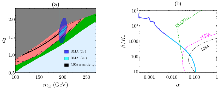
Fig. 3 Real triplet extension of the SM. Panel (a) gives the phase diagram in terms of the triplet mass m_\Sigma and Higgs portal coupling a_2 . The light blue, green, red, and grey areas correspond to singlet step crossover transition, single step first order transition, two step thermal history, and unstable electroweak minimum, respectively. The interior of the black dashed contour corresponds to an EWPT that would complete. The thin black band is the allowed region for a hypothetical LISA observation. The dark (light) ellipses give prospective collider allowed regions for scenarios BMA (BMA'): determination of the triplet mass and Higgs diphoton decay rate (adds a measurement of the neutral triplet decay to two Z bosons). The blue bands in panel (b) show projection of the hypothetical collider allowed parameter space into the plane of GW-relevant inputs. Figures adapted from Ref. [153].
