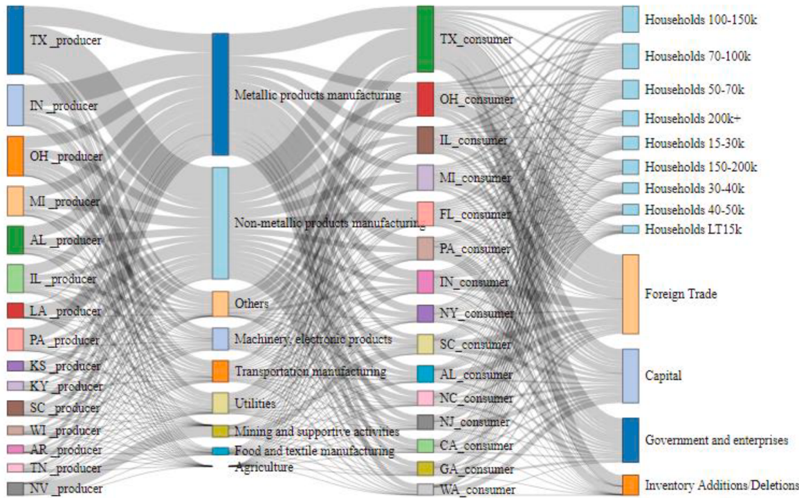
Fig. 5. Flows of embodied TCR from top 15 release producing states to the final consumers in the top 15 consuming states.
