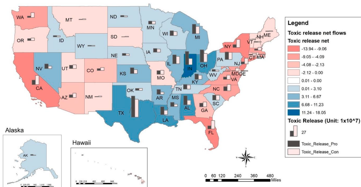
Fig. 1. Production-based and consumption-based TCR and net inflows (red) and outflows (blue) of embodied TCR across states in the US (USA states shapefile: https://www.arcgis.com/home/item.html?id=1a6cae723af14f9cae228b133aebc620 ).
