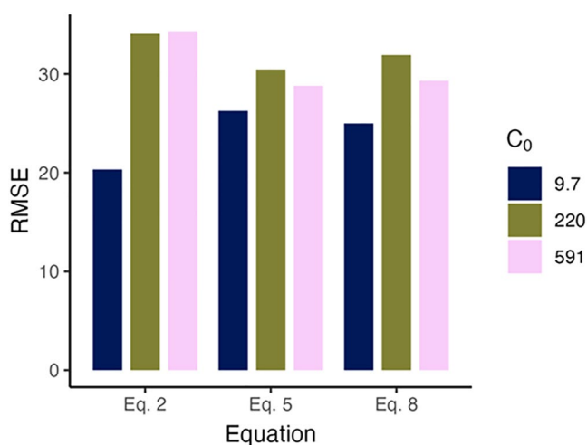
Figure 6. Root mean square error (RMSE) of nonlinear least squares model fit to the 15-min sensor-derived data using the three different C_0 values (9.7 \mu\text{S cm}^{-1} : wet deposition; 220 \mu\text{S cm}^{-1} : baseflow; 591 \mu\text{S cm}^{-1} : soil pore water) for equations where C_0 was included as a non-zero term. RMSE were estimated using 10X-repeated 10-fold cross-validation. 95% confidence intervals are plotted but are too small to be observed at this scale.
