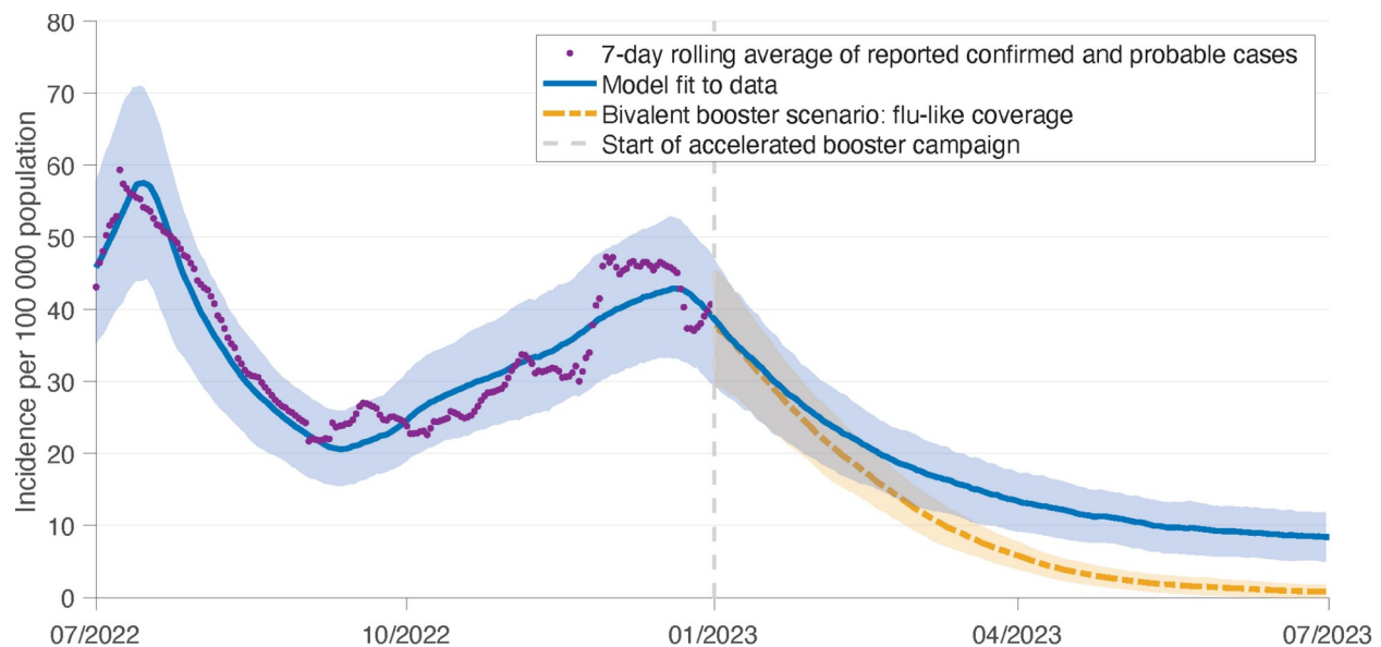
Figure 2: Model fit and projection. Model fit to 7-day rolling average of incidence per 100,000 population with simulated scenarios of bivalent booster vaccination from January 1 to June 20, 2023.
