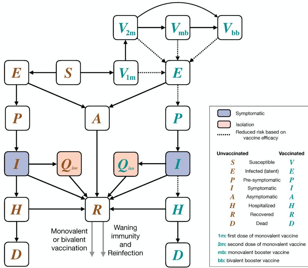
Figure 1. Schematic representation of the model dynamics for infection and vaccination. Infected individuals stay in an exposed period (as part of their incubation period), before becoming infectious and move to the stage of pre-symptomatic or asymptomatic without manifestation of clinical symptoms. Those who develop symptomatic disease after pre-symptomatic stage may practice self-isolation. All symptomatic cases without hospitalization recover after their infectious period. Severe symptomatic cases may be hospitalized and recover or die. Asymptomatically infected individuals recover without self-isolation or hospitalization. Vaccination reduces the risk of infection, symptomatic disease, and severe disease based on the efficacy of each dose in primary series (i.e., monovalent vaccination) and booster (i.e., monovalent or bivalent). Prior to September 15, 2022, booster doses were assumed to be monovalent vaccines. After September 15, 2022, all booster vaccines were assumed to be bivalent. An individual was considered eligible for bivalent booster if the time elapsed since last infection or a previous dose of monovalent vaccines exceeded 2 months.
