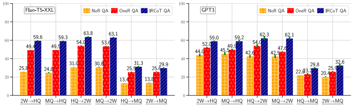
Figure 6: Answer F1 for NoR QA, OneR QA and IRCoT QA using Flan-T5-XXL (Left) and GPT3 (Right) in out-of-distribution (OOD) setting. HQ (HotpotQA), 2W (2WikiMultihopQA), MQ (MuSiQue). The result X→Y indicates prompt demonstrations are from dataset X and evaluation is on dataset Y. IRCoT QA outperforms OneR QA and NoR QA in such an OOD setting.
