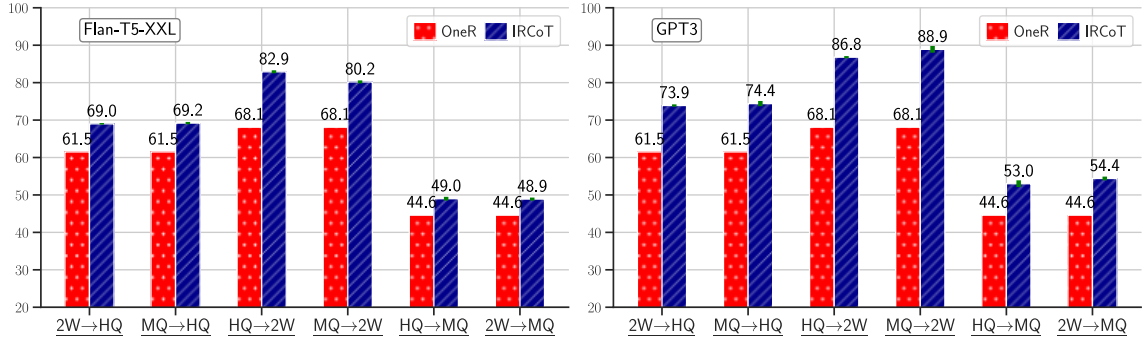
Figure 5: Retrieval recall for OneR and IRCoT using Flan-T5-XXL (Left) and GPT3 (Right) in out-of-distribution (OOD) setting. HQ (HotpotQA), 2W (2WikiMultihopQA), MQ (MuSiQue). The result X→Y indicates prompt demonstrations are from dataset X and evaluation is on dataset Y. IRCoT outperforms OneR in such an OOD setting.
