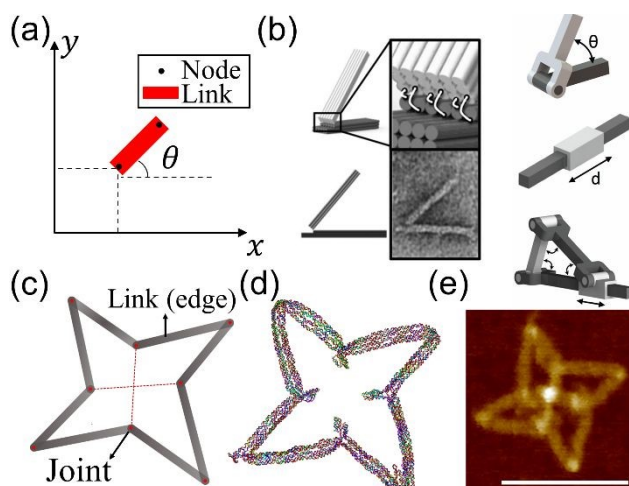
Figure 1. Kinematic mechanisms realized with DNA nanostructures. (a) A planar rigid body (red rectangle) with 3 degrees of freedom (DOF), i.e. , the coordinates x , y , and the angle of inclination \theta . The rigid body is a link. A node shown as black dots is the possible connecting point in the link to other bodies. A link must have at least two nodes. The link can be classified as a binary, ternary, and quaternary link if it has two, three, and four nodes, respectively. (b) A kinematic chain is comprised of links and joints. A joint is a connection between two links at the nodes that allows some degree of motion. An example of common kinematic chains and a nanoscale hinge realized using ssDNA connections (white lines in the inset). The transmission electron microscopy (TEM) image resembles the design. On the right side, angular (top, rotating pin joint), linear (middle, slider joint), and combined motions (bottom) are shown in schematics. (Adapted from ref. 64 with permission. Copyright (2015) National Academy of Sciences) (c)-(e) Architected auxetic metastructures from DNA. (Adapted from ref. 65 with permission. Copyright (2021) Wiley-VCH GmbH) (c) Schematic of a unit cell of a rotating square design composed of links and joints. (d) Coarse-grained molecular dynamics (MD) simulation on the oxDNA platform and (e) Atomic force microscopy (AFM) image of the DNA origami unit. Scale bar: 100 nm.
