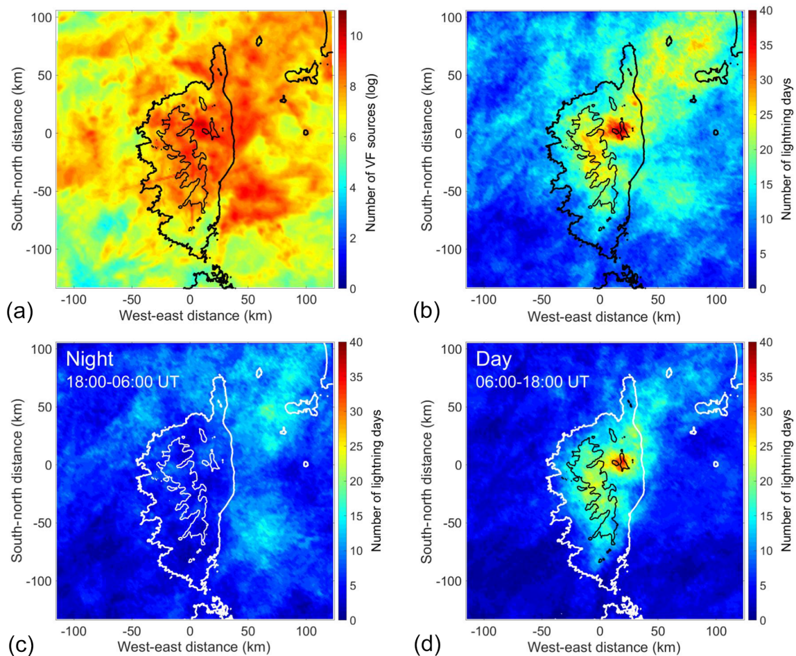
Figure 7. Overall cumulative number of filtered VHF sources in the 240\text{ km} \times 240\text{ km} domain of better detection accuracy centered on Corsica for 2014 to 2016 (a); frequency of lightning days for the overall set of filtered data on the same domain and during the same period (b); frequency of lightning days at night (c) and day (d). A lightning day in a given pixel is defined as a day during which at least five VHF sources are detected in that pixel. Isocontours at 1000 m altitude are indicated by black or white lines inside Corsica.
