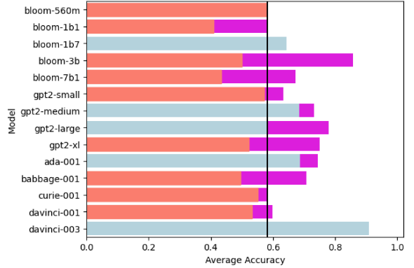
Figure 8: Average accuracy for predicting the label in intr-agent/intr-patient sentences with adjusted thresholds. After this adjustment, all models are at or above majority class accuracy. Magenta segments show increase in performance.
