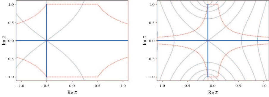
Figure 5. Lax spectrum for the potential q(x) = e^{ix} with minimal period L = 2\pi (blue). Contours \Gamma = \{z \in \mathbb{C} : \text{Im } \Delta_\epsilon(z) = 0\} (black dashed). The curve which bounds the imaginary component of elements in the spectrum |\text{Im } z| = \min\{\|q\|_\infty, \epsilon\|q'\|_\infty/2|\text{Re } z|\} (red dashed). Left. \epsilon = 1 . Right. \epsilon = 0.2 .
