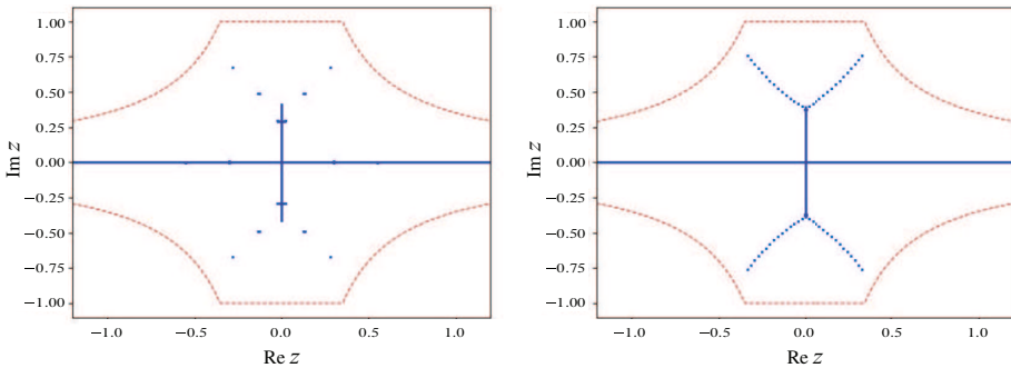
Figure 10. Same as Figure 7 but for the periodic potential q(x; \varepsilon) = \operatorname{dn}(x; m) e^{i 2 \operatorname{dn}(x; m)/\varepsilon} , where m = 0.88 . Left. \varepsilon = 0.2 . Right. \varepsilon = 0.03 .
