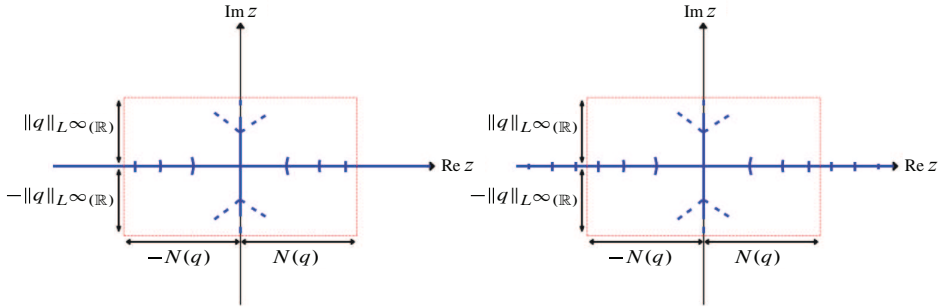
Figure 2. Left. Schematic diagram of the spectrum for a finite-band potential. Right. Schematic diagram of the spectrum for an infinite-band potential.
