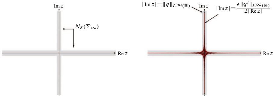
Figure 4. Left. The \delta -neighborhood of \Sigma_\infty (light gray). Right. Bounds on the Lax spectrum for 0 < \varepsilon \leq \varepsilon_* (dark red) with the \delta -neighborhood of \Sigma_\infty (light gray).
