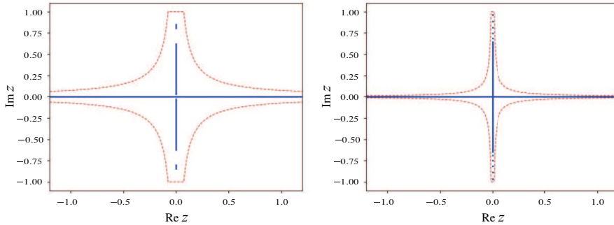
Figure 8. Same as Figure 7, but for the periodic potential q(x) = \text{dn}(x; m) , where m = 0.6 . Left. \varepsilon = 0.5 . Right. \varepsilon = 0.1 .
