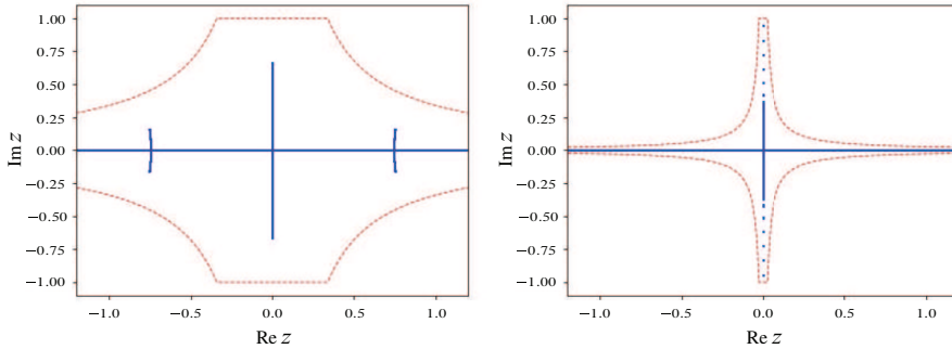
Figure 7. Numerically computed Lax spectrum for the periodic potential q(x) = e^{-\sin^2 x} (blue). The curve which bounds the imaginary component of the eigenvalue |\operatorname{Im} z| = \min\{\|q\|_\infty, \epsilon \|q'\|_\infty / 2\} |\operatorname{Re} z| (dark red dashed). Left. Semiclassical parameter \epsilon = 1 . Right. Semiclassical parameter \epsilon = 0.079 .
