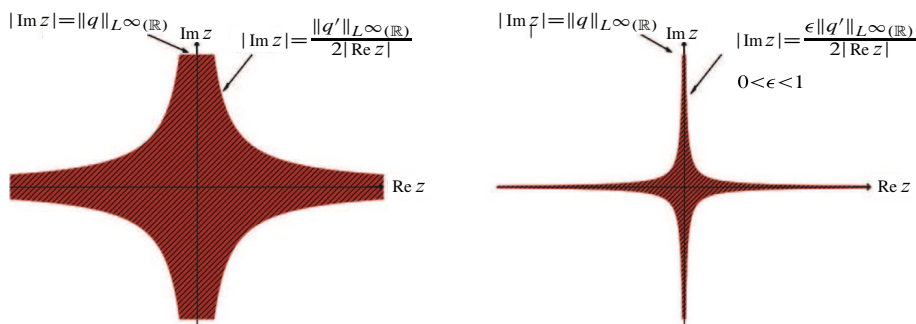
Figure 3. Left. Bounds on the Lax spectrum for \varepsilon = 1 (dark red). Right. Bounds on the Lax spectrum when 0 < \varepsilon < 1 (dark red).
