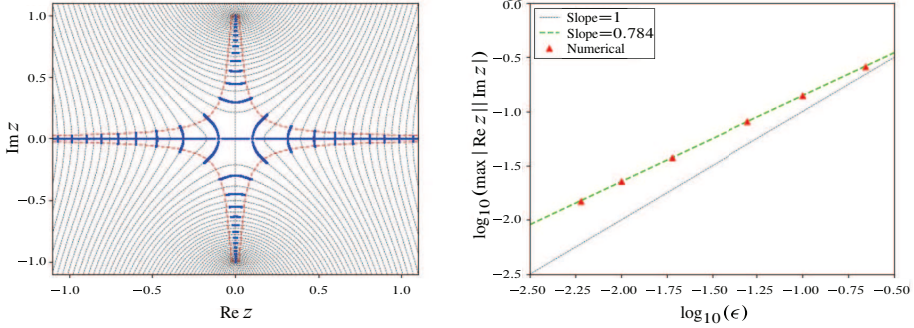
Figure 6. Left. Same as Figure 5 but for the periodic potential q(x) = \text{sgn}(x) with L = 2 , and \epsilon = 0.019 . Right. Convergence of eigenvalues to \Sigma_\infty as \epsilon \downarrow 0 for “sgn” potential. Numerical computation of \max_{v \in [0, 2\pi/L]} |\text{Re } z(v)| |\text{Im } z(v)| as \epsilon \downarrow 0 (red triangles). Least-squares fit through the data points (light green dashed).
