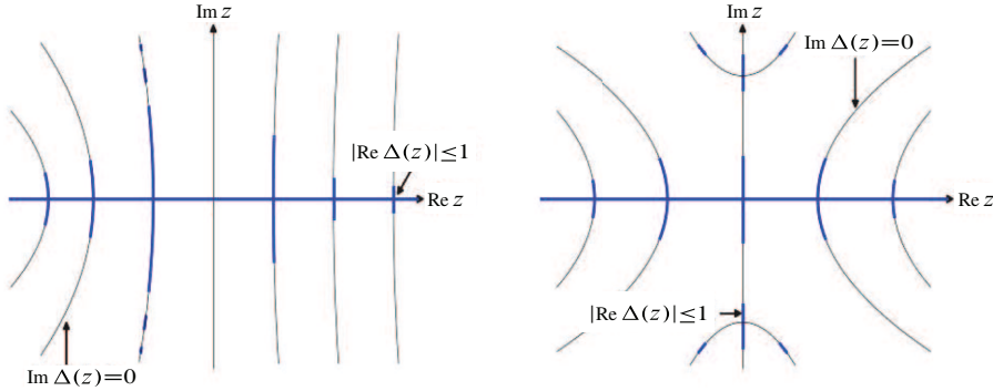
Figure 1. Left. Schematic illustration of the Lax spectrum of the focusing Zakharov–Shabat scattering problem with a generic periodic potential. Right. Schematic illustration of the Lax spectrum of the focusing Zakharov–Shabat scattering problem with a real, even, or odd periodic potential. In these cases elements of the Floquet spectrum come in quartets, i.e., \{z, \bar{z}, -z, -\bar{z}\} (see Lemma 5.1).
