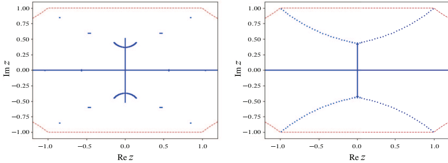
Figure 9. Same as Figure 7 but for the periodic potential q(x; \varepsilon) = e^{i \cos(2x)/\varepsilon} . Left. \varepsilon = 0.22 . Right. \varepsilon = 0.019 .
