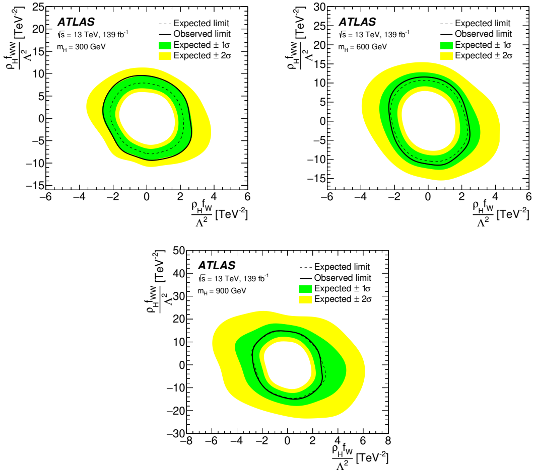
Figure 6. Observed (black solid curve) and expected (black dashed curve) 95% CL upper limits on the production of a heavy Higgs boson as a function of \rho_H f_W / \Lambda^2 and \rho_H f_{WW} / \Lambda^2 for a mass of 300 GeV (top left), 600 GeV (top right) and 900 GeV (bottom). The green (inner) and yellow (outer) bands represent the \pm 1\sigma and \pm 2\sigma uncertainties of the expected limits.
