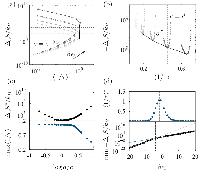
FIG. 3. Speed and dissipation extrema in the parameter space. (a) Entropy dissipated -\Delta_e S/k_B versus speed \langle 1/\tau \rangle averaged over all paths varying \beta\epsilon_b \in [-10, 10] with fixed c = 5 and d = \{0.5, 0.6, 1, 1.5, 4\} . Darker gray indicates larger values of d . Dashed horizontal lines indicate c = e^{-\beta\epsilon_b} for each d . Solid black line connects vertices for different d values. (b) Ensemble level dissipation -\Delta_e S/k_B versus speed \langle 1/\tau \rangle for d \in [1.5, 10] in increments of 0.5 and other parameters fixed at c = 5 and \beta\epsilon_b \in [1, 4] in increments of 1 (darker gray indicates lower value of \beta\epsilon_b ). Dashed vertical lines indicate c = d for each fixed \beta\epsilon_b value. Solid black line connects vertices for different \beta\epsilon_b values. (c) Maximum average speed (bottom) and associated average entropy dissipated -\Delta_e S^*/k_B := -\Delta_e S/k_B|_{\max(1/\tau)} (top) for d \in [0.5, 10] and fixed c = 5 . (d) Minimum entropy dissipated on average (bottom) and associated speed \langle 1/\tau \rangle^* := \langle 1/\tau \rangle|_{\min(-\Delta_e S/k_B)} (top) for \beta\epsilon_b \in [-10, 10] for fixed c = 5 . Dashed lines are exponential trends for \beta\epsilon_b > -\ln c (blue) and \beta\epsilon_b < -\ln c (gray).
