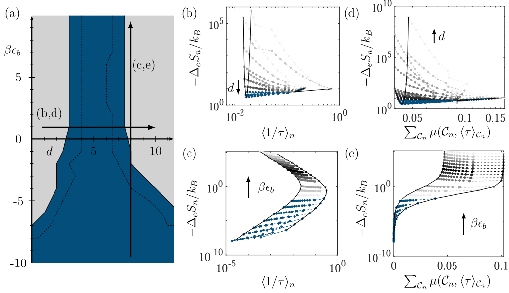
FIG. 2. Model parameters control whether faster paths dissipate more or less entropy on average. (a) Diagram mapping the sign of the slope from -\Delta_e S_n / k_B as a function of \langle 1/\tau \rangle_n for a cross section of the parameter space ( \beta\epsilon_b, d/c = 5 ). For \beta\epsilon_b > 0 , the dissipation increases with speed when c \approx d (blue). For \beta\epsilon_b < 0 , the width of this region grows with increasingly negative \beta\epsilon_b . Arrows indicate the parameter sweeps shown in (b)–(e). (b) When paths are resolved by the number of jumps between the initial and the final states (and averaged), the entropy dissipated to the surroundings -\Delta_e S_n / k_B , can increase or decrease as a function of the mean rate of path completion \langle 1/\tau \rangle_n . The slope is controlled by the current around the cycle, which we tune by sweeping d \in [0.5, 10] in increments of 0.5 at fixed c = 5 and \beta\epsilon_b = 1 . Dissipation increases with the rate of path completion (blue) for c \approx d but decreases sharply when |c - d| \gg 0 (grayscale). Solid lines connecting the slowest paths for the parameter sweep show a parabolic trend (black). (c) Dissipation -\Delta_e S_n / k_B as a function of the mean rate of path completion \langle 1/\tau \rangle_n resolved (averaged) by the path length n . The slope is controlled by sweeping \beta\epsilon_b \in [-10, 10] in increments of 1 with fixed c = 5 and d = 8 . (d) The yield \sum_{C_n} \mu(C_n, \langle \tau \rangle_{C_n}) has the same relationship to the dissipation -\Delta_e S_n / k_B as the speed \langle 1/\tau \rangle_n . (e) Dissipation -\Delta_e S_n / k_B as a function of the yield \sum_{C_n} \mu(C_n, \langle \tau \rangle_{C_n}) resolved (averaged) by the path length n . The yield plateaus above \beta\epsilon_b = 1 .
