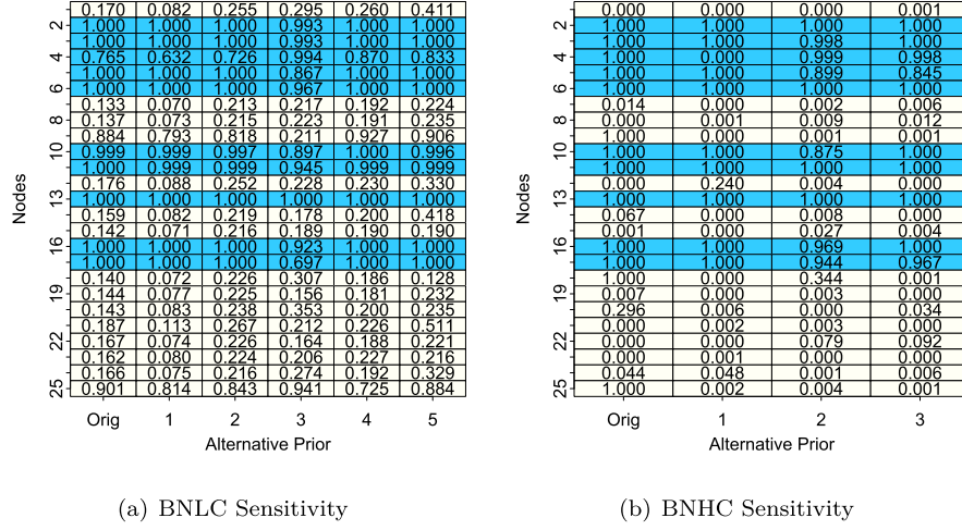
Figure 6: Figure shows P(\xi_k = 1|Data) for BNLC and BNHC under different hyper-parameter combinations in the simulated data for Case 4 (Simulation 1). The first column in each matrix shows the values corresponding to the original prior specification.
