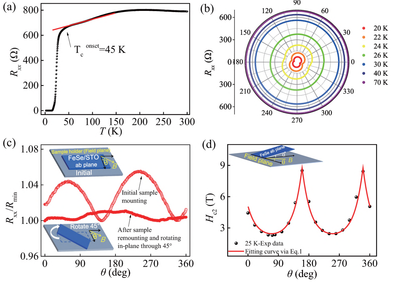
FIG. 3. Absence of anisotropy of in-plane upper critical field of FeSe/STO. (a) Temperature dependent resistance curve of an FeTe capped FeSe film, showing the superconductivity transition with onset T_c around 45 K. The thickness of the film is estimated to be 3 unit cells. (b) Angle-dependence of the in-plane magneto-resistance at various temperatures. (c) Comparison of angle-dependence of the magneto-resistance after rotating and remounting the sample in plane through 45^\circ taken at 18 K and 9 T. The angle position of the two-fold symmetry shifts 70^\circ , and the amplitude becomes smaller, which indicates the two-fold symmetry is not an intrinsic in-plane property of the FeSe film but rather arises from the out-of-plane misalignment. Insets are the schematics of the measurement setup. \theta is the in-plane angle position, and \alpha is the out-of-plane misalignment angle. The magneto-resistance is normalized to the minimum value of the magneto-resistance. (d) Angle-dependence of the critical field extracted from resistance vs field curves at various angles at 25 K. The angle dependence (black dots are the experimental data) can be fit with the 2D Tinkham formula (red curve) by considering a fixed out-of-plane misalignment angle \alpha , confirming that the two-fold symmetry is from the out-of-plane misalignment. Therefore, the in-plane critical field is isotropic within the resolution limit of the measurement.
