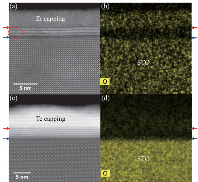
FIG. 2. Atomic resolution HAADF STEM images (a and c) and EDS mapping (b and d) of oxygen of FeSe film with Zr and Te. (a and b) FeSe capped with Zr, (c and d) FeSe capped with Te. The EDS results are on the same scale and the same region as the corresponding STEM images. The Zr layer has an amorphous structure and it partially destroys the crystalline structure of FeSe. The red-circled area does not have as high crystalline quality as other areas. The blue arrows indicate the interface between FeSe film and STO. The red arrows indicate the interface between FeSe film and the capping layer.
