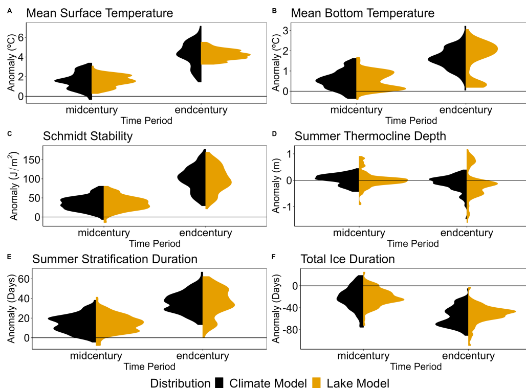
Figure 6 Model-type distributions for mid- and end-century across lake model and climate model uncertainty. Distributions of the model-type mean anomalies of the climate models and lake models under RCP 8.5. These distributions were calculated for (A) mean summer surface temperature (surface temperature), (B) mean summer bottom temperature (bottom temperature), (C) Schmidt stability, (D) thermocline depth, (E) summer stratification duration, and (F) total ice duration during mid-century (2020–2050) and end-century (2069–2099).
