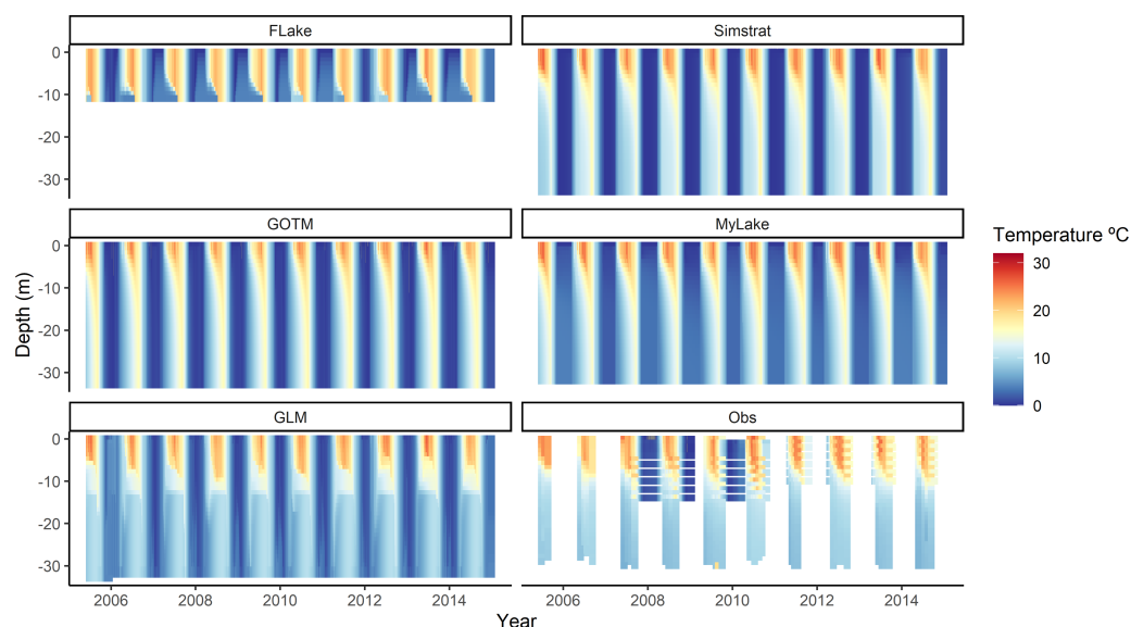
Figure 3 Modeled and observed water column temperatures over the calibration period. Contour plot of whole water column temperature profiles from the surface to the bottom of the lake (with the exception of FLake (surface to 11.0 m) and MyLake (surface to 32.0 m); see ‘Methods: Calibration’) during the calibration period (2005–2015) for each lake model (FLake, GLM, GOTM, Simstrat and MyLake). Observed water temperature data (Obs) for Lake Sunapee, NH are shown in the bottom right panel.
