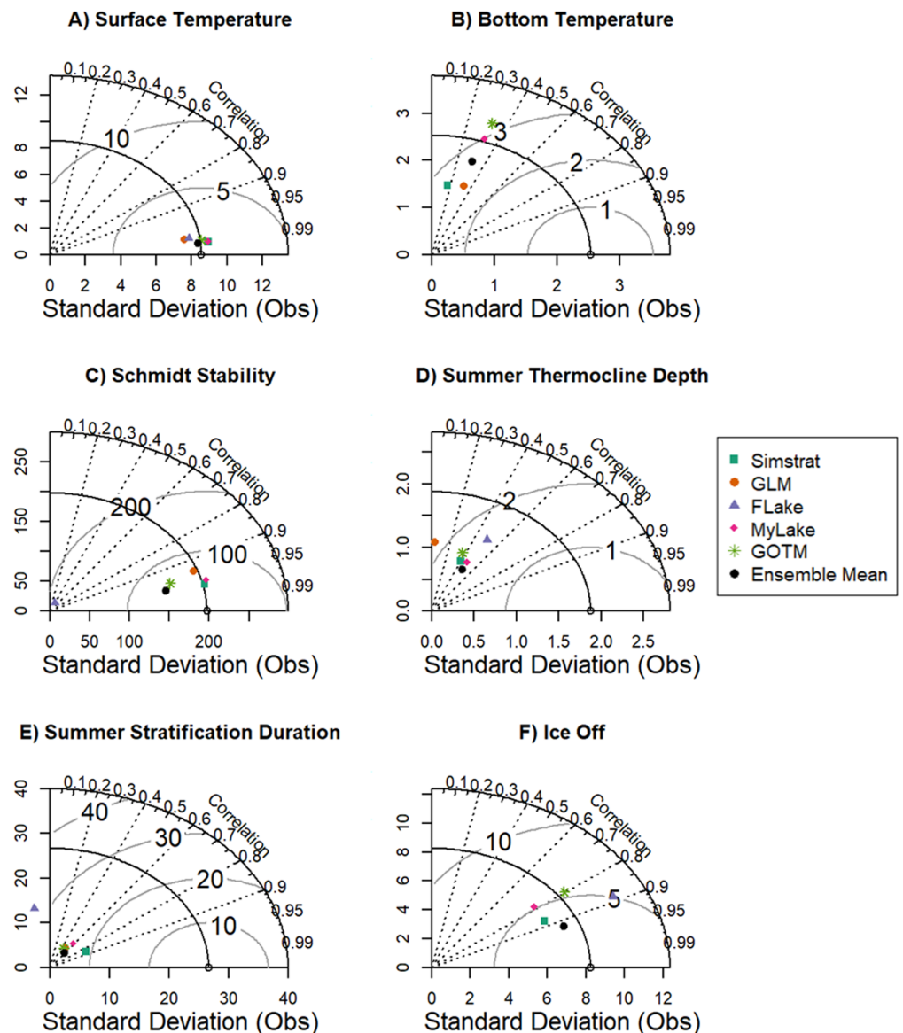
Figure 4 Taylor diagrams showing model performance. Taylor diagrams showing the standard deviation of observations (x-axis) and modeled thermal metrics (y-axis) for Lake Sunapee, NH, USA during 2005–2015. The correlation between observations and modeled output is shown as dotted lines, and root mean squared error (RMSE) between observed and modeled standard deviation is shown as arcs. Correlation ( r ) represents the linear trend between observed and modeled data. Each colored point represents a specific lake model compared with observed data. Thermal metrics include (A) summer surface temperature mean, (B) summer bottom temperature mean, (C) Schmidt stability, (D) summer thermocline depth, (E) stratification duration, and (F) date of ice-off. Summer is defined as June–August. Values to the left of the y-axis (e.g., panel E) represent negative correlation.
