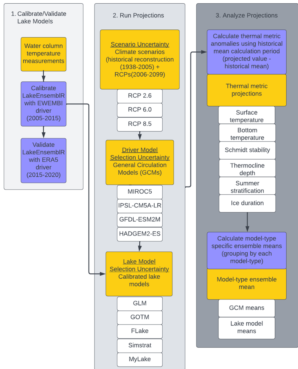
Figure 1 Conceptual workflow representing the methodology used to produce lake thermal projections. Methodological workflow explaining the full projection process starting from Step 1, using observational data to calibrate and validate lake models; Step 2, using a scaffolded approach to create an ensemble of n = 60 model projections which incorporates climate model selection uncertainty (via four GCMs), and lake model selection uncertainty (via 5 lake models); and Step 3, analyze the projection output by first calculating anomalies for each thermal metric using the historical mean calculation period, and then calculating model-type ensemble means (see ‘Methods and Materials: Ensemble means across RCP scenarios’). Yellow boxes represent outputs or inputs in the workflow, while blue boxes represent actions.
