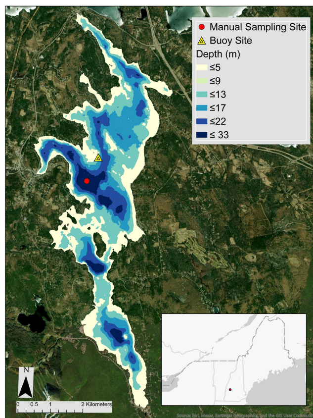
Figure 2 Map of Lake Sunapee, NH. Location and bathymetry of Lake Sunapee, New Hampshire, USA (43.39745°N, 72.05065°W), showing the site of the Lake Sunapee Protective Association GLEON buoy where high-frequency temperature measurements are collected on m intervals to 10 m depth. The red dot denotes a manual sampling location, where monthly water temperature profiles were measured on m intervals to 30 m depth.
