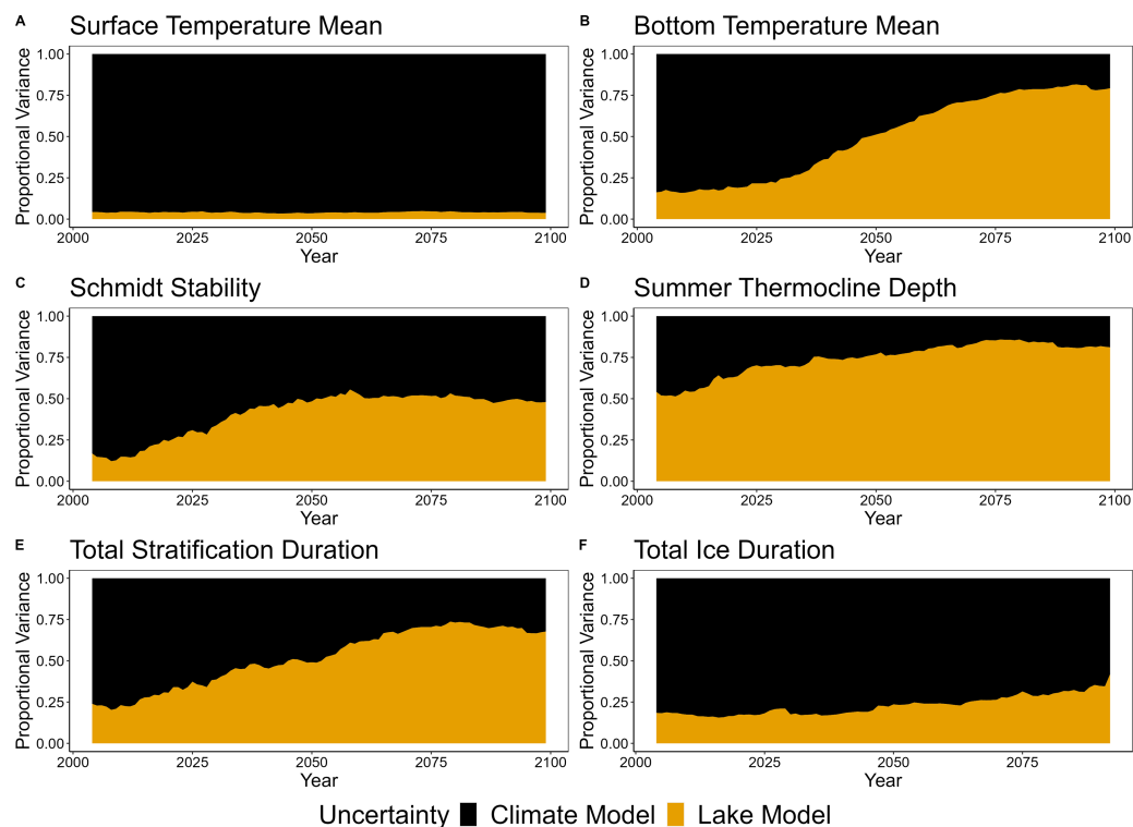
Figure 7 Proportional variance of the contribution of climate model selection uncertainty (black) and lake model selection uncertainty (orange) to total uncertainty. (A) Surface temperature mean (surface temperature), (B) bottom temperature mean (bottom temperature), (C) Schmidt stability, (D) thermocline depth, (E) total stratification duration, and (F) total ice duration from 2006–2099. Proportional variance was calculated for all models using the RCP 8.5 climate scenario.
