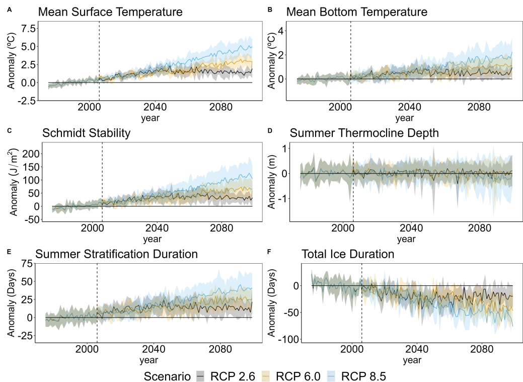
Figure 5 Lake thermal projections through end-century. Projected anomalies for (A) mean summer surface temperature (surface temperature), (B) mean summer bottom temperature (bottom temperature), (C) Schmidt stability, (D) thermocline depth, (E) summer stratification duration, and (F) total ice duration from 2006–2099. The vertical dashed line represents the beginning of the projection time period, with the left of the dashed line representing the historical mean calculation period on which anomalies were based (1975–2005). Each solid line represents the ensemble mean of the lake models under RCP 2.6, 6.0, or 8.5 and each shaded area around the solid lines represents total projection uncertainty under RCP 2.6, 6.0, or 8.5.
