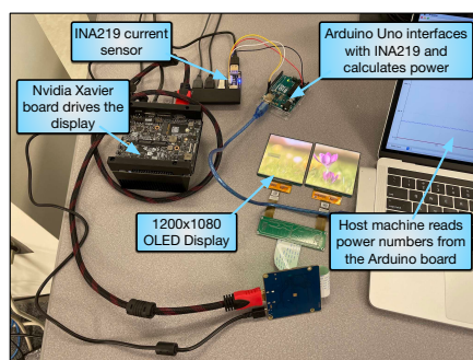
(a) hardware setup
