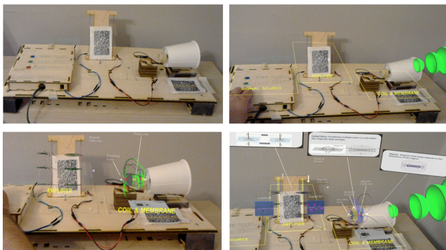
Figure 2. Views of the system under different experimental conditions. Top Left: View without Hololens headset (“Non Hololens” condition). Top Right: Hololens with basic AR, virtually displaying apparatus areas and sound waves (“Hololens Simple” condition). Bottom Left: AR view including magnetic fields in green (visible for a time during the “AR Layered” condition). Bottom Right: AR view including magnetism, electricity, and poster images (“AR Full” condition).
