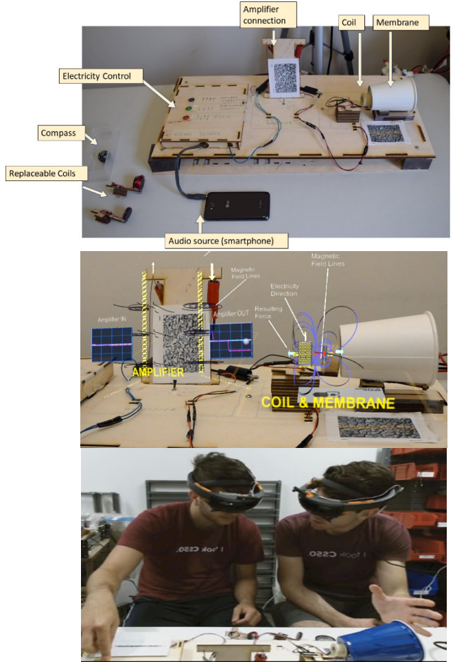
Figure 1. The augmented reality speaker system. Top: physical speaker system. Middle: AR view of the magnetic fields around the coil and the magnet that are generating the sound waves. Bottom: two users interacting with the speaker activity using AR headsets.
