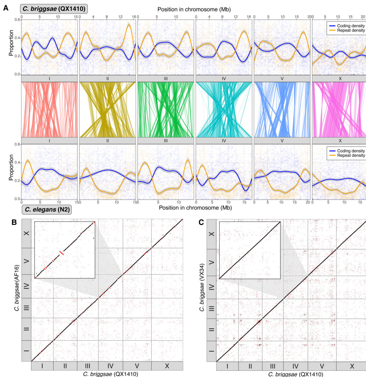
Fig. 1. —High-quality reference genomes for two C. briggsae strains. (A) Comparison between the C. briggsae QX1410 and C. elegans N2 reference genomes. Repeat density and protein-coding gene density per 10 kb windows are shown. Repeats were identified de novo using RepeatModeler2. Solid lines represent LOESS smoothing functions fitted to the data. Relative positions of 10,387 one-to-one orthologs are shown as lines joining the two density plots. (B) Whole-genome alignment of AF16 to the QX1410 reference genome generated using nucmer. Alignments shorter than 1 kbp are not shown. Alignments in the reverse orientation are highlighted in red. Inset: chromosome IV showing multiple regions between AF16 and QX1410 that are in different orientations. (C) Whole-genome alignment of VX34 to the QX1410 reference genome generated using nucmer. Alignments shorter than 1 kbp are not shown. Alignments in the reverse orientation are highlighted in red. Inset: the same chromosome IV region as in (B) showing a largely collinear alignment.
