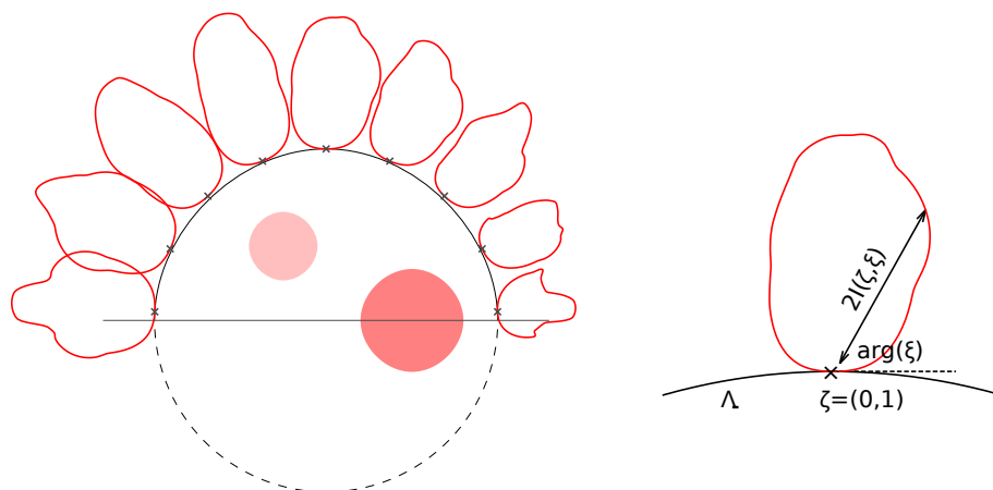
Figure 4. Measurement data I|_{\Lambda_+} . The red curves depict the outflow I(\zeta, \xi) in polar coordinate centered at \zeta (cross symbol \times ) and radius 2I(\zeta, \xi) . The outflow through \zeta = (0, 1) is magnified in the right figure. The red inclusions show the highly absorbing regions given as a priori information (the medium is assumed to be known).
