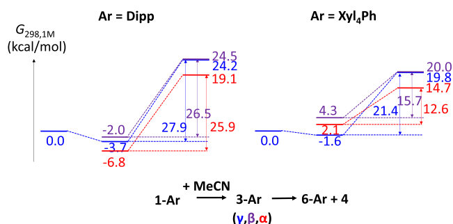
Figure 4. Relative Gibbs energies for the QM/MM calculations of the chelate ring opening by MeCN in 1-Ar,γ and of the Pd–C homolytic bond cleavage in 3-Ar,α/β/γ, yielding 4-α/β/γ and 6-Ar (Ar = Dipp, left; Xyl 4 Ph, right).
