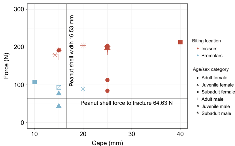
Fig. 4. Maximum in vivo bite forces and gapes for each animal colored by initial fracture location for peanut shell. Point shape indicates age/sex category. The plot includes lines for average width and force to fracture for the nut shell. Tufted capuchins used postcanine dentition to initially fracture peanut shells until their maximum in vivo bite forces and gape exceeded the width and force needed to initially fracture peanuts shells using an FLS-II tester by 30–40%.
