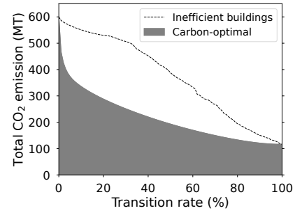
Fig. 9. Carbon emissions at varying levels of transition to electric heat pumps from gas-based heating while jointly optimizing for carbon emissions reduction and targeting energy inefficient buildings.
